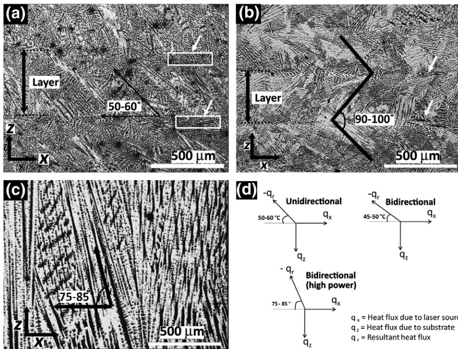
Fig. 4 – Optical micrographs showing the dendrites orientation and layer demarcation in (a) unidirectional deposition (B1), and (b) bidirectional deposition (B2), both built using similar process parameters, (c) high power condition (B3), and (d) schematic illustrations of the heat flux directions (not to scale).
