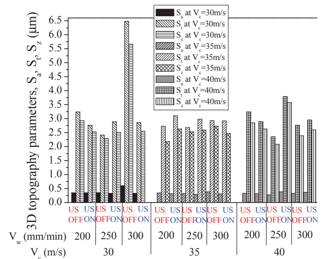
Fig. 4. 3D topographical parameters of ground workpiece surfaces
