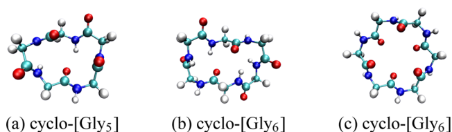
Figure 5. Selected conformers of cyclo-[Gly 5 ] and cyclo-[Gly 6 ] optimized with the AMBER ff03 potential in water.
