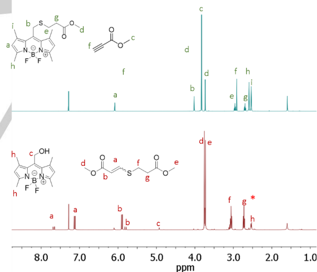
Figure 2. ^1\text{H NMR} spectra of compound 1 (1 eq.) and methyl propiolate (3 eq.) in water/acetonitrile ( v/v = 1/4 ) before (top) and after irradiation (bottom) with green light ( \lambda = 530\text{ nm} , I = 30\text{ mW cm}^{-2} ) for 5 h. After irradiation, the solutions were lyophilised, during which methyl propiolate was evaporated together with the solvent, before being dissolved in \text{CDCl}_3 for NMR analysis.
