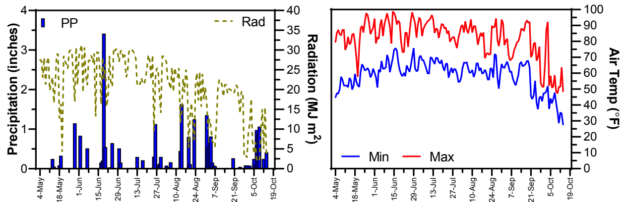
Figure 1. Daily precipitation (blue bars, inches), global radiation (dashed line, MJ/m 2 ) on the left, and daily air temperature (minimum = blue line, and maximum = red line) on the right, for the 2018 corn-soybean season at Scandia, KS.
