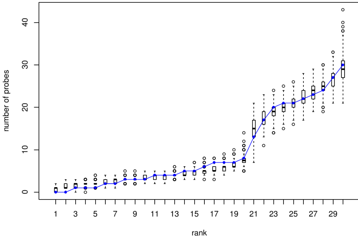
Klun data: glm model
