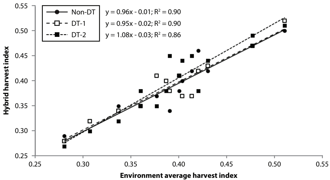
Figure 2. Regression of individual hybrid harvest index on mean harvest index for three hybrids in 18 environments in Kansas during 2014 and 2015.
