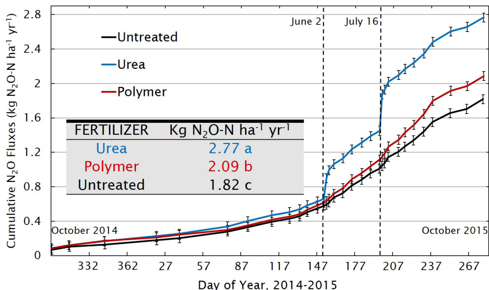
Figure 4. Cumulative fluxes of N 2 O-N from plots treated with urea, polymer-coated urea, and untreated. Vertical dashed lines represent fertilization dates.
