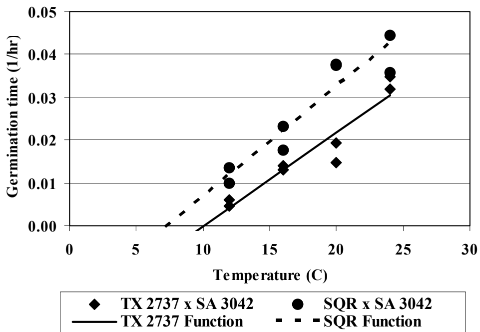
Figure 6. Heat requirements for seed germination can be calculated from time required for germination when incubated at a range of temperatures. Seeds with SQR as male parent accumulated heat units more rapidly than seeds with TX 2737 as male parent.
