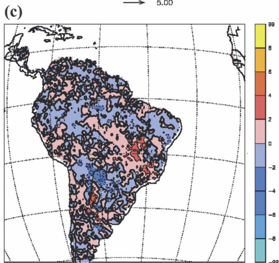
FIG. 10. Same as in Fig. 8, but from experiment 0.5*SM+SST .
