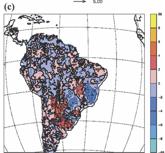
FIG. 11. Same as in Fig. 8, but from experiment 0.5*SM-TOPO .
