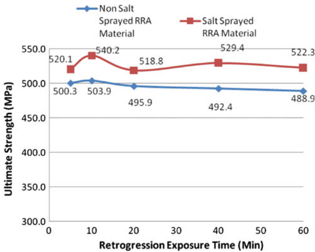
Fig. 3 Ultimate strength vs. retrogression exposure time in RRA material with retrogression exposure temperature at 200 °C after reaging process 2
