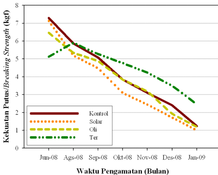
Gambar 4. Kekuatan putus benang polyamide selama penelitian. Figure 4. Breaking strength of polyamide twine during experiment.
