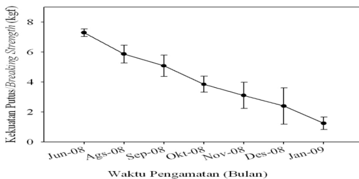
Gambar 3. Kekuatan putus benang polyamide selama penelitian. Figure 3. Breaking strength of polyamide twine during experiment.
