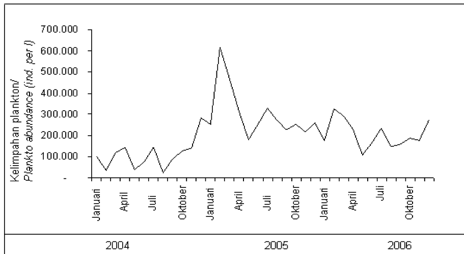
Gambar 12. Kelimpahan plankton di Waduk Ir. H. Djuanda menurut waktu pengamatan (bulan dan tahun). Figure 12. Plankton abundance according to the observation time (months and years) in Ir. H. Djuanda Reservoir
