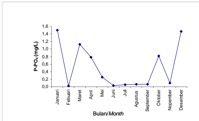
Gambar 10a. Hubungan antara rata-rata konsentrasi P-PO 4 (mg per l) di Waduk Ir. H. Djuanda terhadap waktu pengamatan (bulan). Figure 10a. Relationship between average of concentration P-PO 4 (mg per l) in Ir. H. Djuanda Reservoir and observation time (month).
