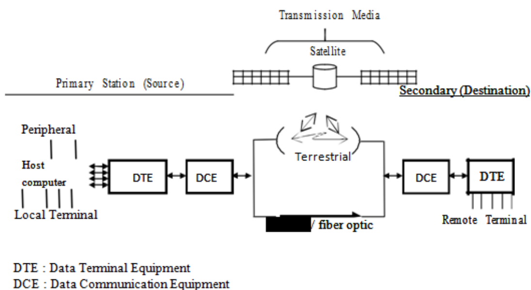
Fig 1. The simple block diagram of communication network
