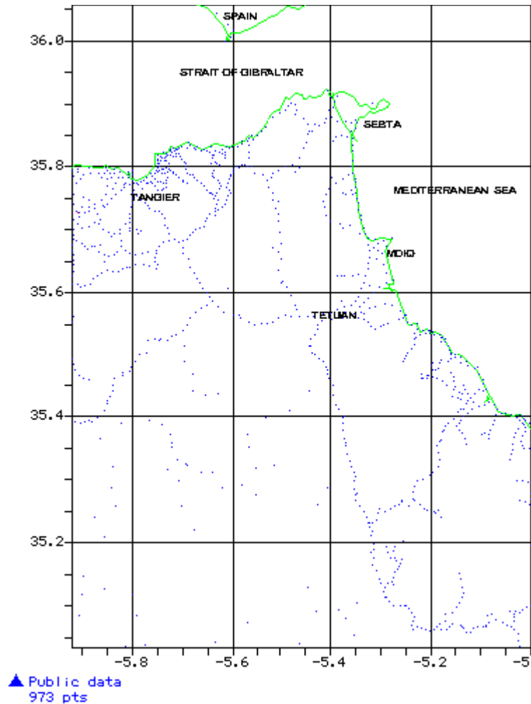
Fig. 3. Data gravity reference map (BGI,2005)
