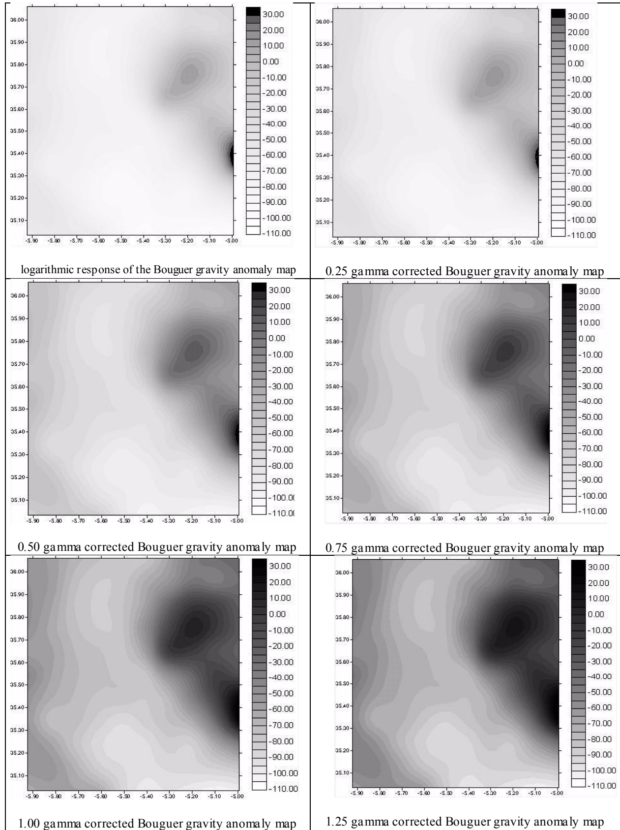
Fig. 6. Logarithmic and gamma corrected Bouguer anomaly gravity maps
