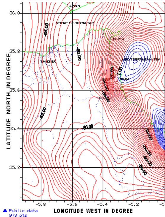
Fig. 4. Bouguer anomalies map of the area of Tangier-Tetuan (interval contour 3 mGal, blue contours correspond to positive Bouguer anomalies)
