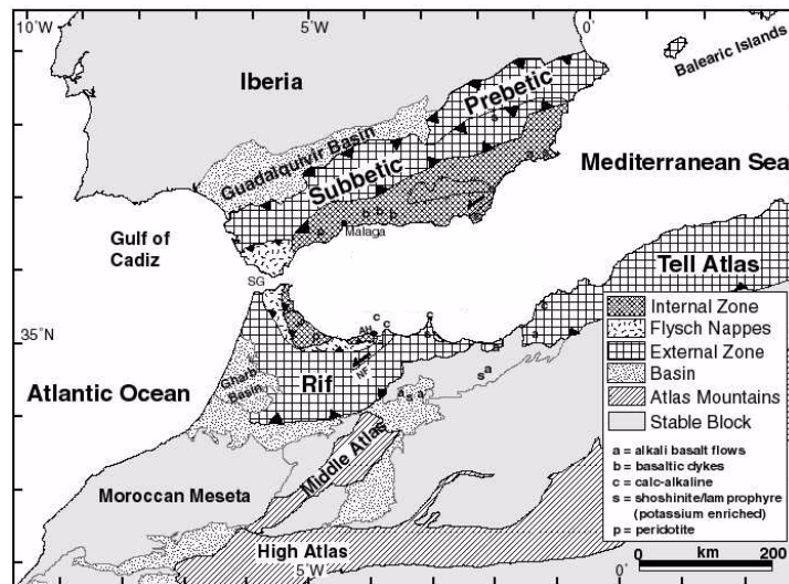
Fig. 2. Principal geological features of the Riffian field
