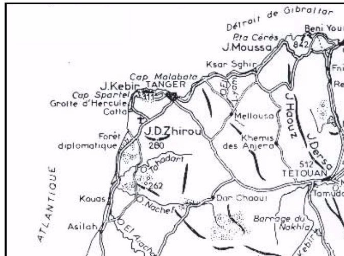
Fig. 1. Situation of the study area
