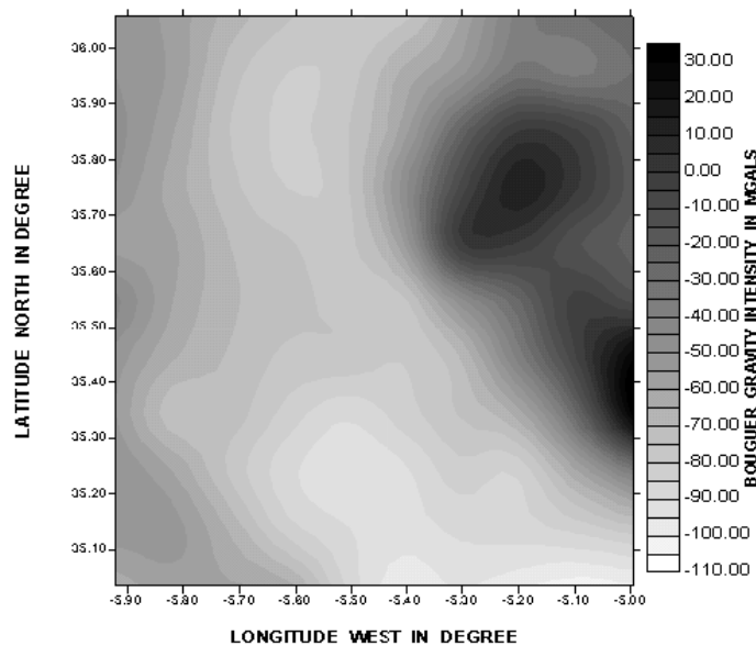
Fig. 5. Bouguer gravity anomalous zones of the area of Tangier-Tetuan
