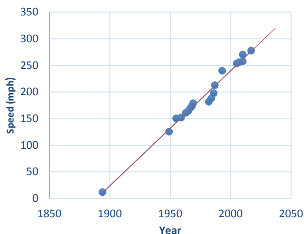
Figure 1 – Trend of production car top speed
