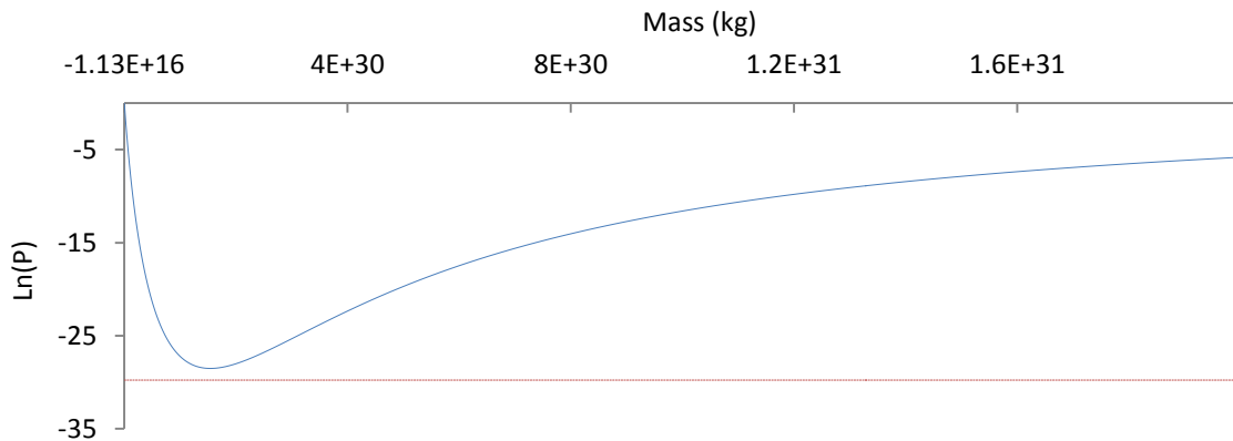
Figure 2. The plot of Eqn. 6 is shown as the blue line and the limit of the LISM is shown as the red line. At no value of M does the solar pressure become low enough to be halted by the LISM.
