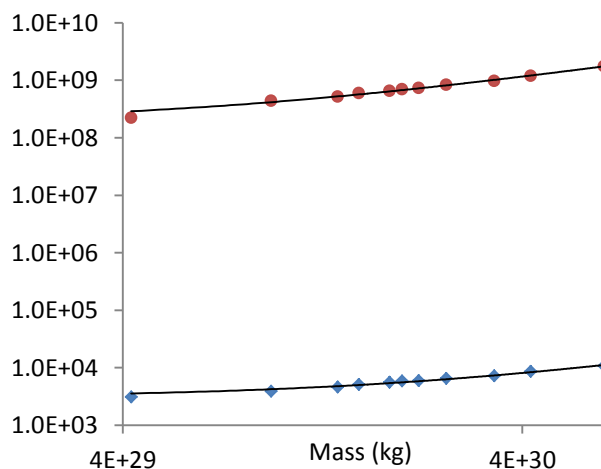
Figure 1. A graph showing the relationship between mass and temperature (K) (blue) and mass and radius (m) (red) for the data in Tab. 1.
