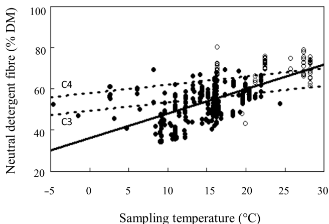
Figure 2. The linear relationship between forage-neutral detergent fibre (NDF) content and temperature ( ^{\circ}\text{C} ) at the time of sampling. The filled circles are C3 species and the open circles are C4 species ( P < 0.05 ). The dotted lines represent best fit lines for C3 ( \text{NDF} = 0.4T + 49 ) and C4 species ( \text{NDF} = 0.4T + 58 ). The continuous line represents the best fit line for all species excluding other factors included within the LME model ( \text{NDF} = 1.1T + 36 ).
