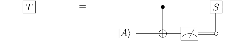
Figure 5: The gadget used to replace a T-gate [91]. |A\rangle = \frac{1}{\sqrt{2}}(|0\rangle + e^{i\pi/4}|1\rangle) are magic states [92].
