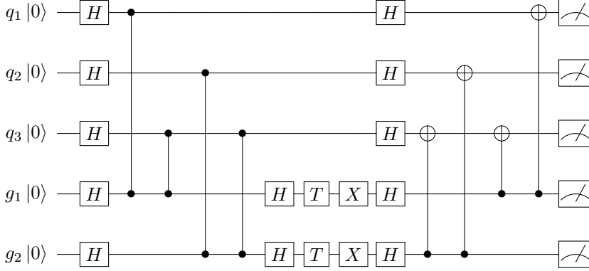
Figure A1: Circuit which implements the MBQC pattern of Figure 2. Measurements have been delayed until the end. The final CX gates perform the necessary adaptive corrections.
