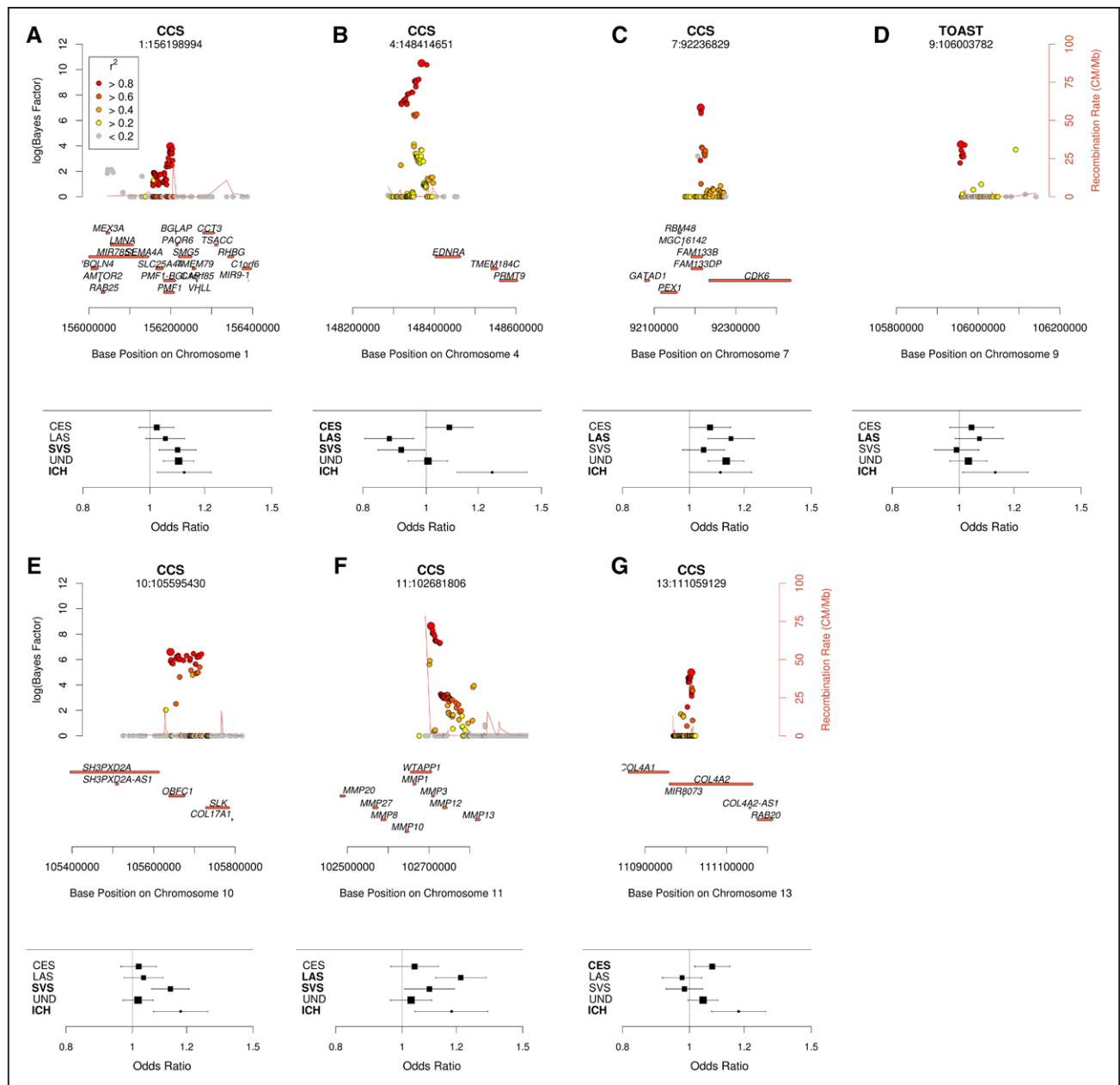
Figure 2. Local plots showing associations with regions conferring risk of ischemic and hemorrhagic stroke and odds ratios for all stroke subtypes. A, 1q22 region; (B) Endothelin receptor type A region; (C) Cyclin dependent kinase 6 CDK6 region; (D) Long Intergenic Non-Protein Coding RNA 1492 region; (E) SH3 And PX Domains 2A region; (F) Matrix metalloproteinase 12 region; and (G) COL4A2 collagen type IV alpha 2 chain region. Results are presented for the classification system in which the locus showed strongest significance. Stroke subtypes in bold indicate those included in the best fitting model and, therefore, predicted to be influenced by the lead genetic variant, based on Bayesian model selection. CCS indicates causative classification of stroke system; CES, cardioembolic stroke; LAS, large artery atherosclerotic stroke; SVS, small vessel stroke; ICH, intracerebral hemorrhage; TOAST, Trial of Org 10172 Acute Stroke Treatment Classification System; and UND, stroke of undetermined cause.
