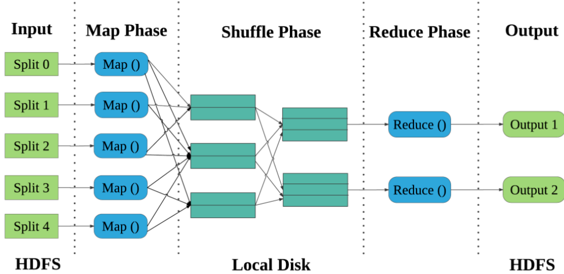
Figure 2. The Structure of MapReduce Model
