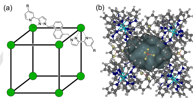
Figure 1. The host cages [Co_8L_{12}]^{16+} , abbreviated as H ( R = H ; soluble in MeCN) and H^w ( R = CH_2OH ; soluble in water). (a) A sketch emphasising the cubic array of Co(II) ions and the disposition of a bridging ligand; (b) a view showing the cavity space (volume 409 \text{ \AA}^3 ).
