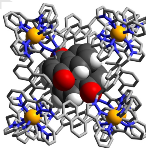
Figure 8. Structure of the complex \text{H}\cdot(\mathbf{12})_2 with the host cage H in wireframe but the stacked pair of guests 12 shown space-filling.
