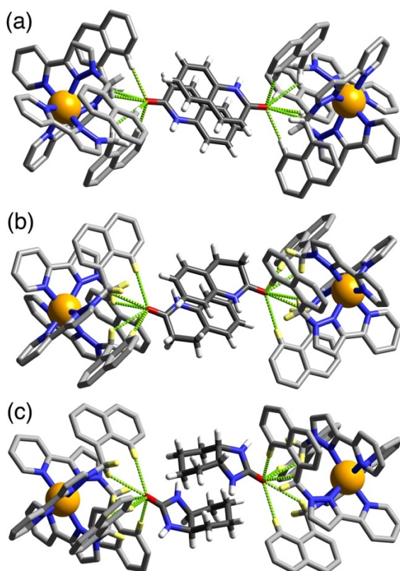
Figure 7. Views of parts of the structures of the \text{H}\cdot\text{G}_2 complexes of H with guests (a) 7 , (b) 8 , and (c) 9 , showing in each case the H-bonding interactions between the carbonyl unit of each guest and the H-bond donor pockets on the host. In every case the two guests lie astride an inversion centre. \text{CH}\cdots\text{O} distances in the H-bonding pockets span the range 2.49 – 2.76 Å (for 7 ); 2.48 – 2.79 Å (for 8 ); and 2.60 – 2.85 Å (for 9 ).
