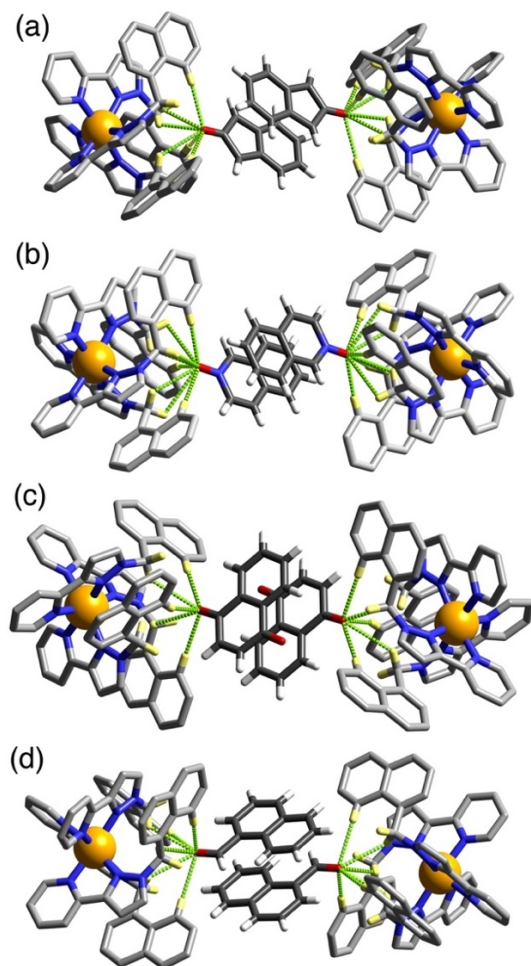
Figure 9. Views of parts of the structures of the \text{H}\cdot\text{G}_2 complexes of H with guests (a) 10 , (b) 11 , (c) 12 and (d) 13 , showing in each case the H-bonding interactions between the carbonyl unit of each guest and the H-bond donor pockets on the host. In every case the two guests lie astride an inversion centre. \text{CH}\cdots\text{O} distances in the H-bonding pockets span the range 2.42 – 2.77 Å (for 10 ); 2.50 – 2.77 Å (for 11 ); 2.51 – 2.98 Å (for 12 ); 2.56 – 2.84 Å (for 13 ).
