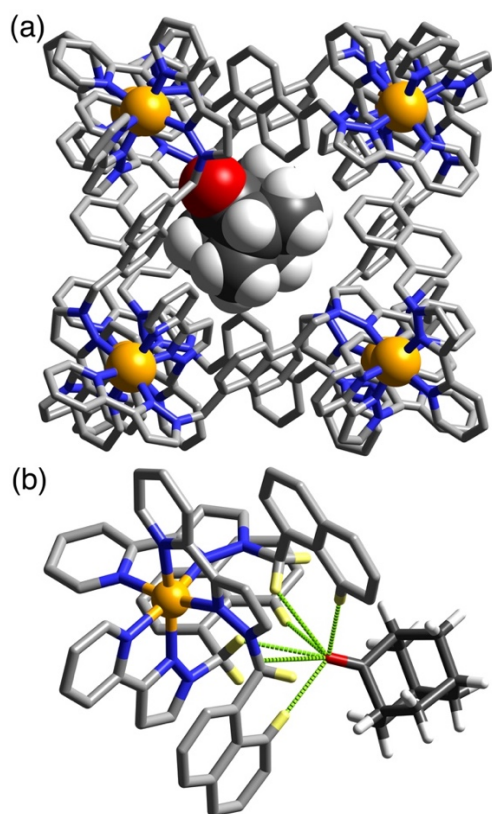
Figure 2. (a) Structure of the complex H•1 with the host cage H in wireframe but the guest 1 shown space-filling. A fractional-occupancy water molecule also present in the cavity is not shown. (b) H-bonding interactions in the structure of the H•1 complex between the carbonyl unit of the guest and the convergent set of CH protons on the host (CH...O distances, 2.46 – 2.98 Å).
