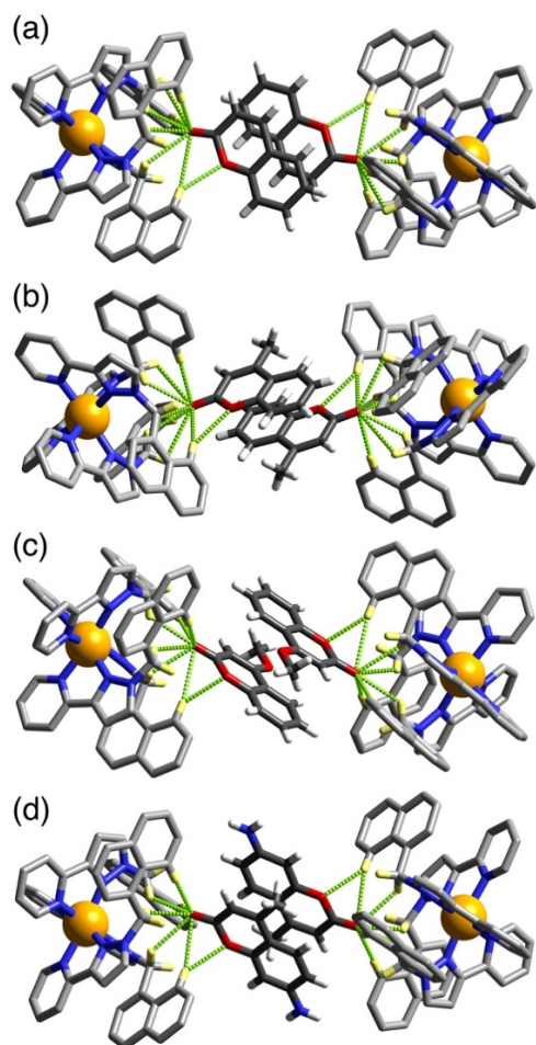
Figure 5. Views of parts of the structures of the \text{H}\cdot\text{G}_2 complexes of H with guests (a) 3 , (b) 4 , (c) 5 and (d) 6 , showing in each case the H-bonding interactions between the carbonyl unit of each guest and the H-bond donor pockets on the host. \text{CH}\cdots\text{O} distances in the H-bonding pockets span the range 2.46 – 2.92 Å (for 3 , major disorder component); 2.42 – 2.98 Å (for 4 , major disorder component); 2.50 – 2.80 Å (for 5 , major disorder component); 2.48 – 2.83 Å (for 6 ). In every case the two guests lie astride an inversion centre.
