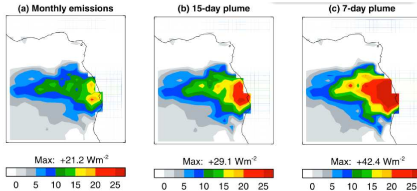
FIGURE 3. (a) HadGEM2 modeled cloudy-sky shortwave aerosol direct radiative effect in \text{W m}^{-2} , averaged over 1–8 August 2006 at 9:30 local time for cloud cover larger than 0.3. The mean aerosol DRE over clouds for this experiment averaged over the
