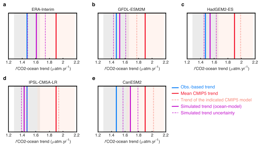
Figure 7. North Atlantic f\text{CO}_2\text{-ocean} trends (thick magenta line) and uncertainty due to interannual variability in the atmospheric forcing (dashed magenta lines) returned from the ocean-only simulations that were forced with (a) ERA-Interim, (b) GFDL-ESM2M, (c) HadGEM2-ES, (d) IPSL-CM5A-LR, and (e) CanESM2 daily surface conditions. The orange dashed line in (b)–(e) shows the trend value for the corresponding Coupled Model Intercomparison Project Phase 5 (CMIP5) model (e.g., in b, the dashed orange line is the f\text{CO}_2\text{-ocean} trend calculated from the GFDL-ESM2M model, as in Table 1). All simulated trends are here model-drift corrected (see Text S4; Figures S13 and S14). The blue and red lines correspond to the observation-based f\text{CO}_2\text{-ocean} trend and the CMIP5 model-mean, respectively. The gray and orange shadows correspond to the 3\sigma returned by the CMIP5-based multiple linear regression analysis and by the intermodel spread.
