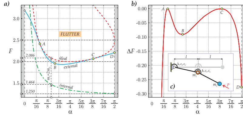
Fig. 10 (a) The (dimensionless) follower force F , shown as a function of the (transformed via \cot \alpha = m_1/m_2 ) mass ratio \alpha , represents the flutter domain of (dashed/red line) the undamped, or ‘ideal’, Ziegler pendulum [110] and the flutter boundary of the dissipative system in the limit of vanishing (dot-dashed/green line) internal and (continuous/blue line) external damping. (b) Discrepancy \Delta F between the critical flutter load for the ideal Ziegler pendulum and for the same structure calculated in the limit of vanishing external damping. The discrepancy quantifies the Ziegler’s paradox due to external (air drag) damping [132].
