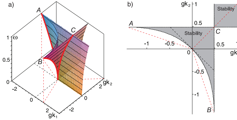
Fig. 7 (a) Stability domain (18) of the Brouwer's rotating vessel and (b) its cross-section at \omega = 0.7 [64, 65].
