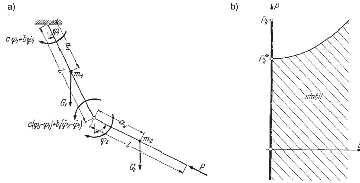
Fig. 9 Original drawings from Ziegler's work of 1952 [146]: (a) double linked pendulum under the follower load P , (b) (bold line) stability interval of the undamped pendulum and (shaded area) the domain of asymptotic stability of the damped pendulum with equal coefficients of dissipation in both joints. If b = 0 we have no dissipation and the system is marginally stable for P < P_k .
