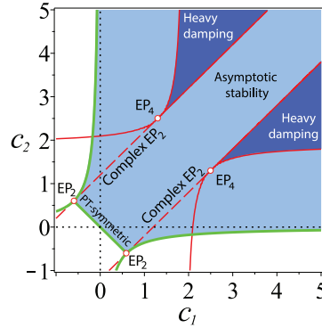
Fig. 8 Domain of asymptotic stability of the damped Brouwer's rotating vessel in the plane of the damping coefficients for gk_1 = 1 , gk_2 = 1 , and \omega = 0.3 [65, 66].
