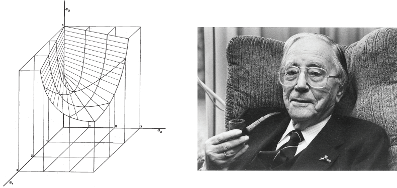
Fig. 11 Original drawing (left) from the 1956 work [25] of Oene Bottema (right), showing the domain of the asymptotic stability of the real polynomial of fourth order and of the two-dimensional non-conservative system with Whitney's umbrella singularity discussed in the sequel. The ruled surface (called V in the text) is given by equation (37).
