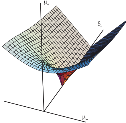
Fig. 14 The critical surface for the damped combination resonance in (\mu_+, \mu_-, \delta_+) space, where \mu_+ = \mu_1 + \mu_2 , \mu_- = \mu_1 - \mu_2 , \delta_+ = \delta_1 + \delta_2 . The parameters \delta_1 and \delta_2 control the detuning of the frequencies \omega_1 and \omega_2 , the parameters \mu_1 and \mu_2 the damping of the oscillators. The self-intersection of the surface with the Whitney umbrella singularity is along the \delta_+ axis [49].
