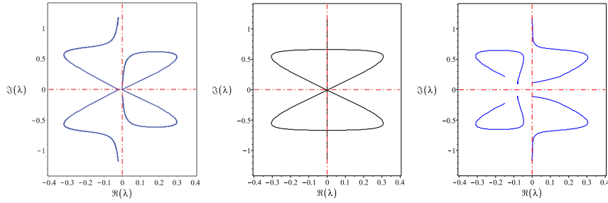
Fig. 5 Paths of the eigenvalues in the complex plane for (left) viscous Maclaurin spheroids with \mu = \frac{\nu}{a_1^2 \sqrt{\pi G \rho}} = 0.002 , (centre) Maclaurin spheroids without dissipation, and (right) inviscid Maclaurin spheroids with radiative losses for \delta = 0.05 . The collision of two modes of the non-dissipative Hamiltonian system shown in the centre occurs at the Riemann critical value e \approx 0.9529 . Both types of dissipation destroy the collision and destabilize one of the two interacting modes at the Meyer-Liouville critical value e \approx 0.8127 .
