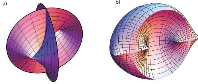
Fig. 13 (a) The Plücker conoid in the unfolding of a semisimple 1 : 1 resonance has a pair of Whitney umbrellas [50]; (b) two pairs of Whitney umbrellas on the boundary of the stability domain of a general 4-degrees-of-freedom dynamical system near a semisimple 1 : 1 resonance [51].
