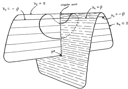
Fig. 12 Whitney's umbrella, lowest dimensional case with 3 parameters [138, 139].
