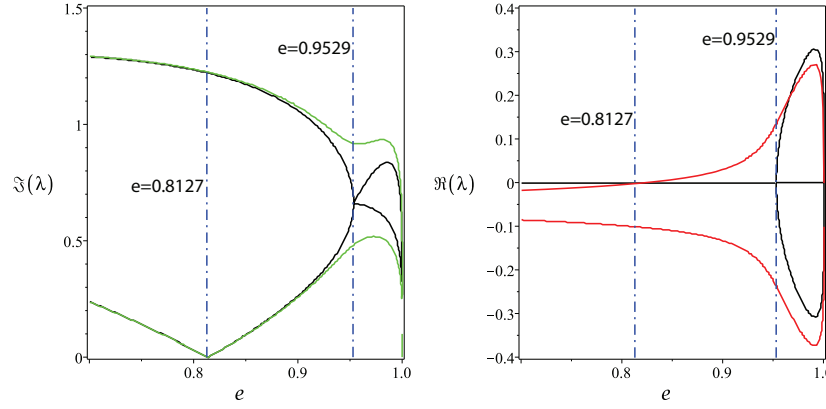
Fig. 4 (Left) Frequencies and (right) growth rates of the (black lines) inviscid Maclaurin spheroids and (green and red lines) viscous ones with \mu = \frac{\nu}{a_1^2 \sqrt{\pi G \rho}} = 0.01 . Viscosity destroys the gyroscopic stabilization of the Maclaurin spheroids on the interval 0.8127.. < e < 0.9529.. , which is stable in the inviscid case [31, 33, 106].
