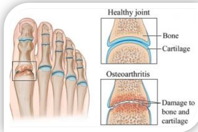
Figure 14: Health joint and Osteoarthritis at joint [26]
