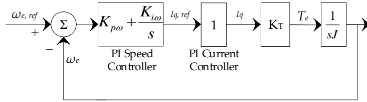
Figure 5.14. Simplified speed control loop of PMSM – Motoring mode
