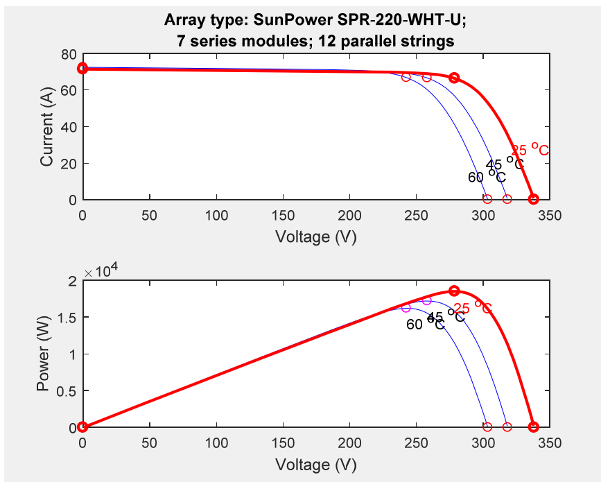
Figure 6.12. I-V and P-V characteristics of 12x7 PV arrays at 1000 ( W/m^2 ) & specified temperatures
