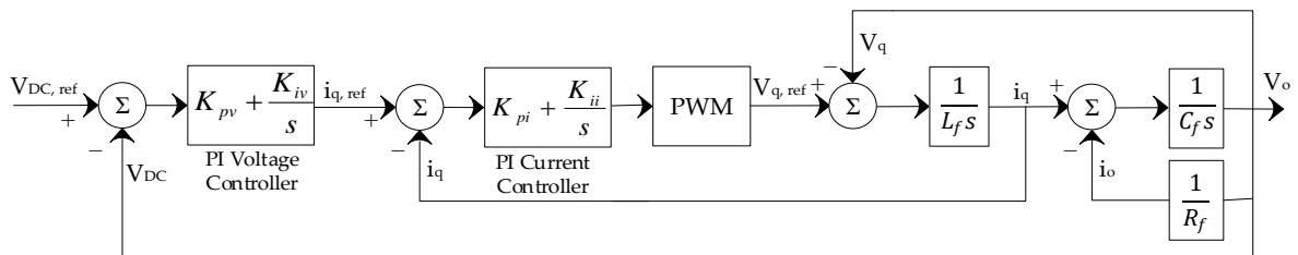
Figure 5.15. Cascaded voltage and current loop of PMSM – Generating mode
