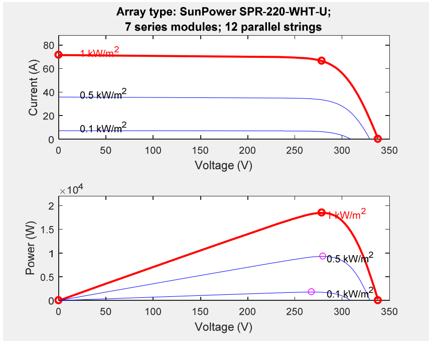
Figure 6.11. I-V and P-V characteristics of 12x7 PV arrays at 25°C and specified irradiances
