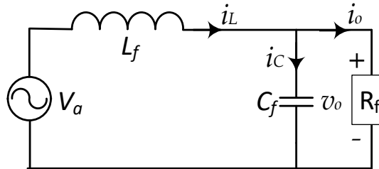
Figure 5.12. Inverter and LC filter equivalent circuit
