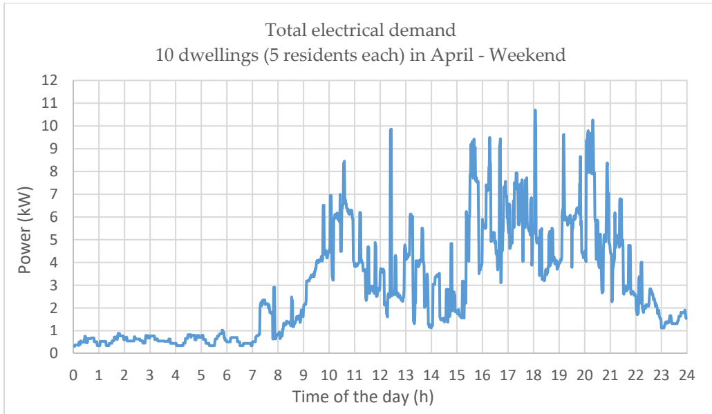
Figure 6.20. 24 hour total electrical demand – Profile 2
