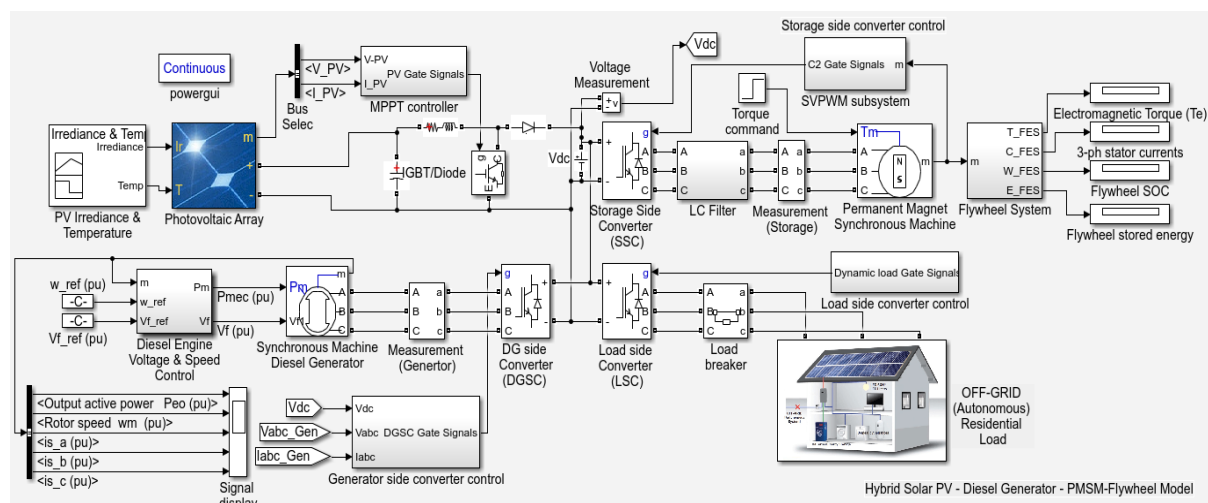
Figure 6.15. An autonomous PV-DGEN-FESS hybrid model connected to a residential load
