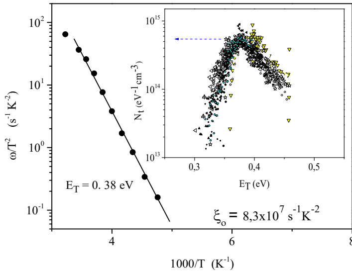
Figure 6 Arrhenius plot of the frequency response data for the most commonly observed in-gap defect state seen in this study, at 0.38 eV. The inset shows the distribution for the corresponding density of trap states. This data is for the most efficient device from the trial, Cell 120/20, having 120 nm of CdS and processed with CdCl 2 for 20 mins.
