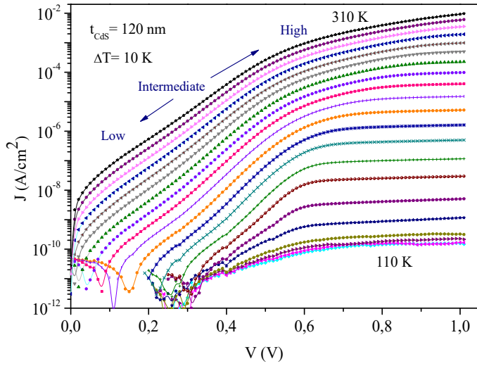
Figure 1. Log plot of dark forward bias J - V:T data for CdS/CdTe Cell120/20, the highest efficiency device from the study. The curves show behaviour that is typical for most of the devices studied: there is ‘roll over’ contact limitation to the current at the relatively ‘high’ voltages. Curves in the ‘intermediate’ voltage range show complex temperature dependent behaviour discussed in the text. At ‘low’ voltages, and for all data recorded below 200K, there is a separate current transport regime.
