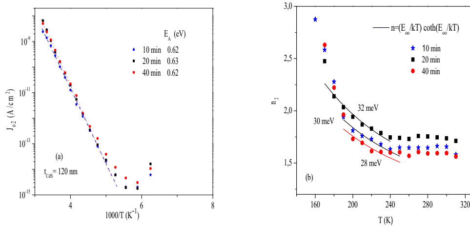
Figure 3. Plots of (a) \log J_{02} vs. 1/T and (b) n_2 vs. T for CdTe/CdS solar cells having 120 nm of CdS and processed for 10, 20 and 40 minutes. As for the other devices, thermally activated processes dominate the reverse bias saturation current behaviour down to \sim 200 K. Fits to n(T) for tunnelling assisted interface recombination are good for 200 < T < 240 K.
