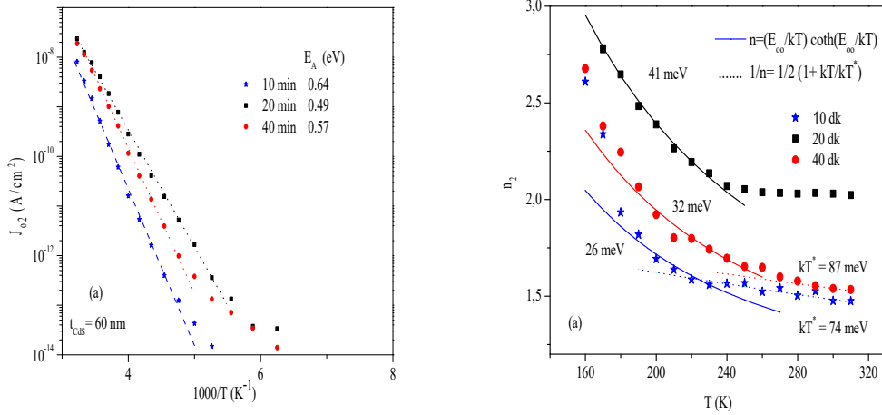
Figure 2. Plots of (a) \log J_{02} vs. 1/T and (b) n_2 vs. T for CdTe/CdS solar cells having 60 nm of CdS and processed for 10, 20 and 40 minutes. J_0 shows thermally activated behaviour down to 180 – 200K. In (b) fit lines are shown below 240K for n(T) for the case of tunnelling assisted interface recombination. Above 240K, n(T) for two of the devices could be fitted using the model for SRH recombination through a continuous distribution of band-tail states
