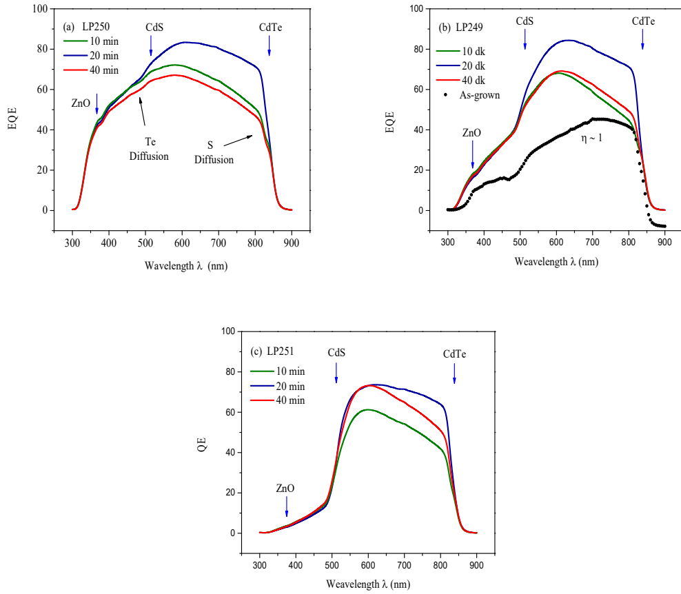
Figure S1. External quantum efficiency (EQE) - \lambda characteristics for CdS/CdTe cells fabricated with 60, 120 and 240 nm of CdS and CdCl 2 processing times of 10, 20 and 40 mins. The absorption edges for CdS and CdTe are shifted slightly by interdiffusion to form CdS y Te 1-y and CdTe 1-x S x intermixing layers at the CdS/CdTe junction interface. The band gap values for these compositions were estimated from [\hbar\nu (1-EQE)]^2 - \hbar\nu and [\hbar\nu EQE]^2 - \hbar\nu characteristics, [20 - 22]. The x -axis intercepts of the linear parts of the plots were used to calculate the amount of intermixing from the Vegard relations E_g(x) = 1.74x^2 - 1.01x + 1.51 eV [20] and E_g(y) = 2.4y + 1.51(1 - y) - 1.8y(1 - y) eV [23] for CdTe 1-x S x and CdS y Te 1-y solid solutions, respectively. Values of the fractions of S in CdTe and Te in CdS are given in table S1 – there was no detectable systematic variations in the level of interdiffusion with either the CdS thickness or the CdCl 2 processing time.
