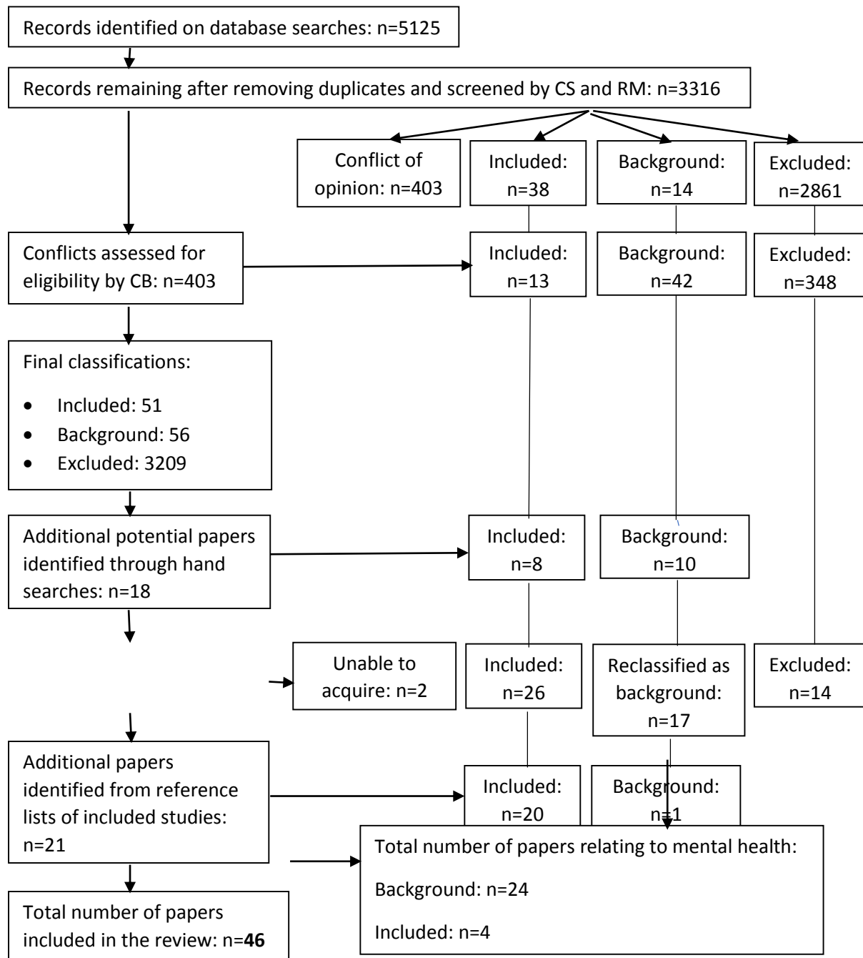
Figure 1: PRISMA diagram
