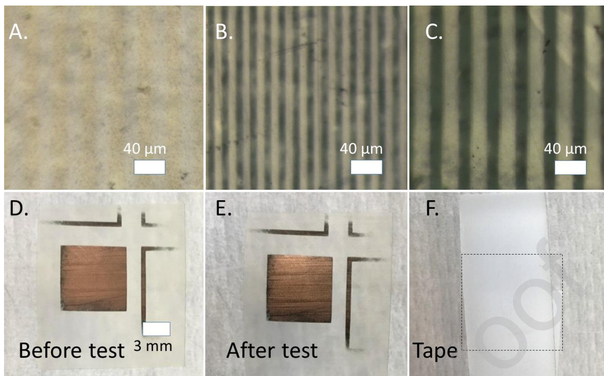
Figure 4 – A) PEI ULTEM 1000B by using spinach extract treatment and photopatterning, revealing 20 μm wide tracks. B) Patterned and electroless copper plated sample with 10 μm wide tracks, and 20 μm (C). D) Electroless copper plated sample before the tape test, and after (E). F) Image of the tape revealing that no copper has been removed.
