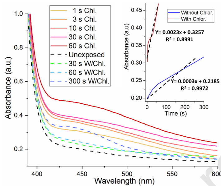
Figure 7 – UV/VIS absorbance of photopatterned samples with spinach extract (Chl) and without (W/Chl.) exposed at different times. The insert is the absorbance measured at 450 nm.
