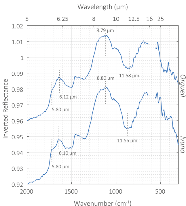
Fig. 6. MIR spectra for CI1 chondrites. The blue spectra reflect the PSF petrologic type I.1. Spectra are inverted and offset for clarity. Both spectra show similar features to the CMs; near 6 \mu\text{m} , a Christiansen feature (CF) and a transparency feature (TF). These features are highlighted. The gap in the spectra is a region of low signal-to-noise due to the beamsplitter.
