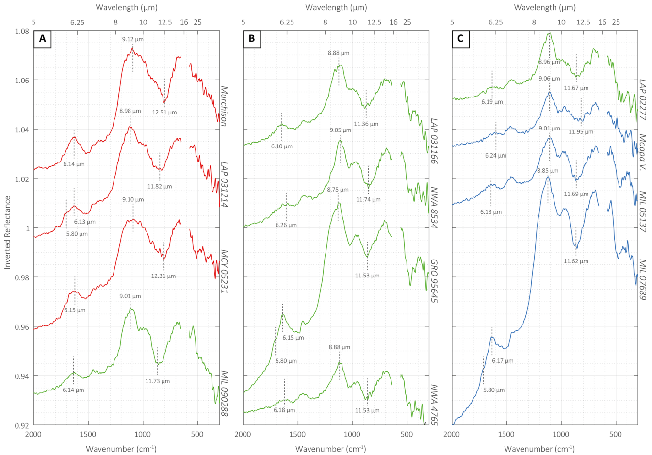
Fig. 5. MIR spectra for (A) Murchison, LAP 031214, MCY 05231, and MIL 090288; (B) LAP 031166, NWA 8534, GRO 95645, and NWA 4765; and (C) LAP 02277, Moapa Valley, MIL 05137, and MIL 07689. Red spectra are PSF petrologic type 1.5, green 1.2, and blue 1.1. Spectra are inverted and offset for clarity. All spectra show a feature near 6 \mu\text{m} due to combination and overtone vibrations of phyllosilicates, a Christiansen feature (CF) related to the optical constants of the constituent mineralogy, and a transparency feature (TF) in a region of optical transparency in fine-grained samples. These features are highlighted. The gap in the spectra is a region of low signal-to-noise due to the beamsplitter.
