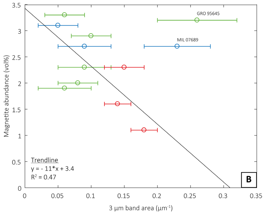
Fig. 8. Fe-cronstedtite abundance versus 3 \mu\text{m} band area (A) and magnetite abundance versus 3 \mu\text{m} band area (B) for the CM1/2 and CM1 chondrites. The 3 \mu\text{m} band area is correlated with both increasing with increasing Fe-cronstedtite and decreasing with increasing magnetite. The two outliers with larger band areas and lower Fe-cronstedtite abundances are MIL 07689 and GRO 95645, which are highly weathered and contain Fe-(oxy)hydroxides (see text for details).
