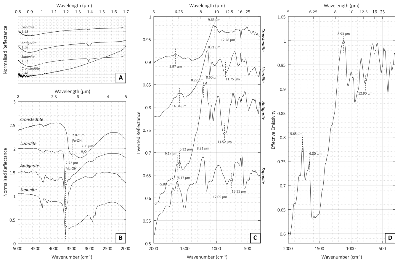
Fig. 2. A) VNIR spectra for the serpentinite minerals cronstedtite, lizardite, and antigorite and the smectite mineral saponite. Spectra are normalized to unity at 0.8 \mu\text{m} and offset for clarity. Ratios are calculated as the reflectance at 1.65 \mu\text{m} divided by the reflectance at 1.05 \mu\text{m} are included on the figure. B) The 3 \mu\text{m} feature for the serpentinite phyllosilicates cronstedtite, lizardite, and antigorite and the smectite phyllosilicate saponite. Spectra are normalized to unity at 2.3 \mu\text{m} and offset for clarity. Features of interest are marked on the figure. C) MIR spectra for the serpentinite phyllosilicates cronstedtite, lizardite, and antigorite and the smectite phyllosilicate saponite. Spectra are inverted and offset for clarity. Features of interest are marked on the figure. D) The emissivity spectrum of San Carlos Olivine in the MIR wavelength ranges. Features of interest are marked on the figure.
