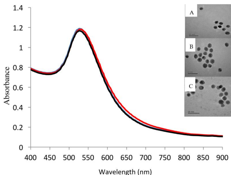
Figure 1. UV-vis absorption spectrum of modified Au NPs. Inset: TEM images (scale bar 20 nm) (black: (A) GPDCALNNC-, blue: (B) GPG-EN-PEG 4 -LA-, and red: (C) C/G-capped Au NPs).
