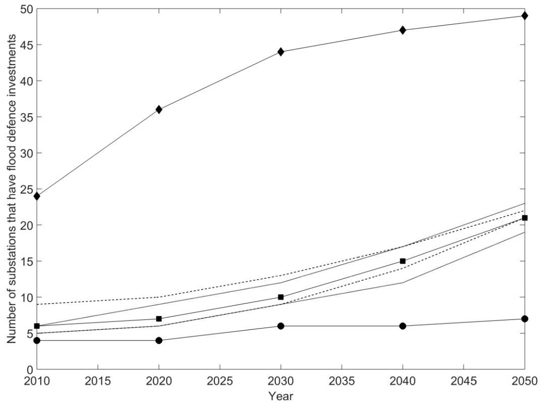
Figure 12: Number of substations undertaking flood defence investments up to 2050. For DCF methodology (black circles) and real option valuation methodology (black squares). The effect in varying the depth damage curve (dotted lines), discount rate (dashed line) and log-normal probability distribution (black diamonds) is also shown.
