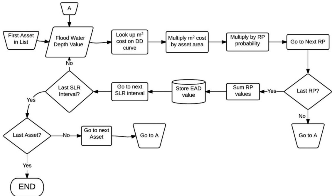
Figure 6: Flow chart showing the process in calculating EAD for each grid cell containing an infrastructure asset.
