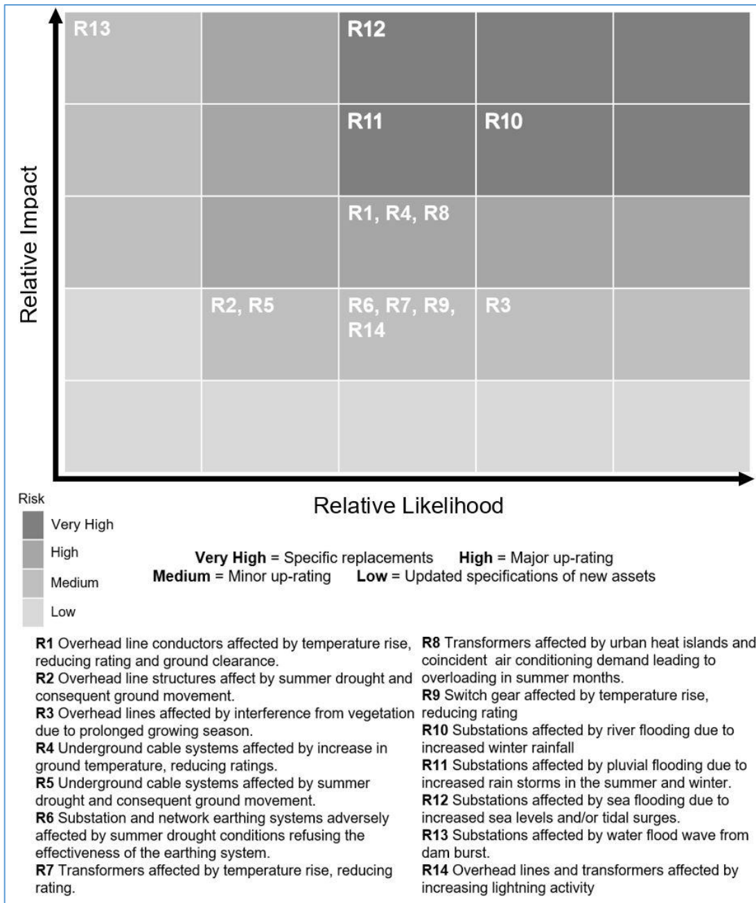
Figure 1: Risk matrix showing biggest projected risks to energy infrastructure up to 2100. This assumes that no adaptation measures are taken and that the high emissions scenario of United Kingdom Climate Projections 2009 (UKCP09) at the 90% probability level is the climate scenario that is realised (Energy Network Association, 2009).
