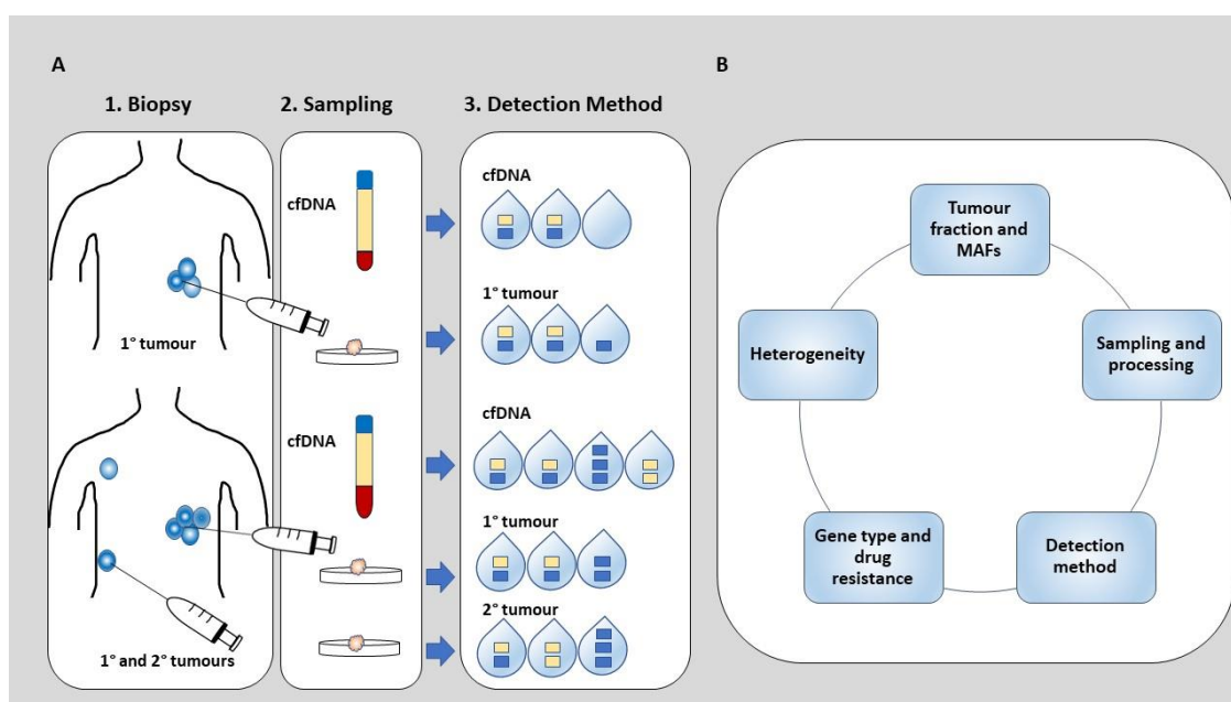
Figure 1. Analysis of cfDNA and tumour tissue in patients with solid tumours: (A) tissue biopsies and cfDNA samples of patients with primary or metastatic tumours are processed for detection of specific somatic genomic alterations (SGAs). The concordance rate between cfDNA and primary tumour or
