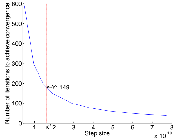
Fig. 6. The number of iterations to achieve convergence.
