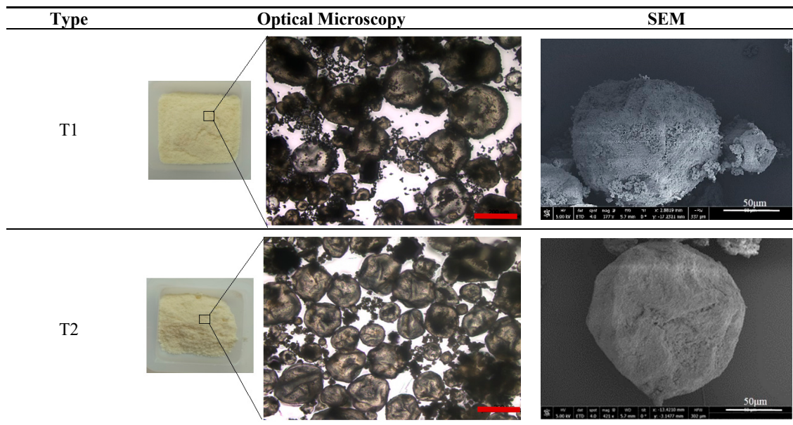
Figure 2. Optical and SEM images of the T1 and T2 microcapsules used in this study.
