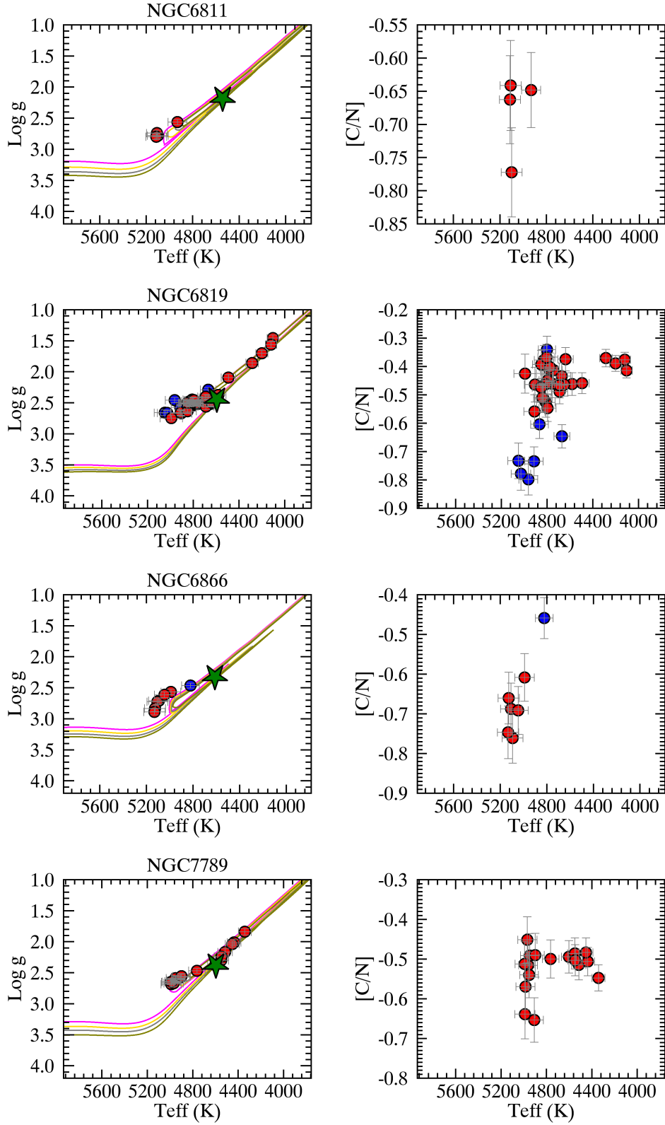
Fig. A.8. \log g - T_{\text{eff}} diagram with PISA isochrones (left panel) and [C/N] abundance vs. T_{\text{eff}} (right panel) of the APOGEE clusters. Symbols and colours are the same as in Fig. 4. The isochrones are 0.8, 1.0, 1.2, and 1.4 Gyr, 1.7, 1.9, 2.1, and 2.3 Gyr, 0.7, 0.8, 0.9, and 1.0 Gyr, and 1.0, 1.2, 1.4, and 1.7 Gyr, respectively.
