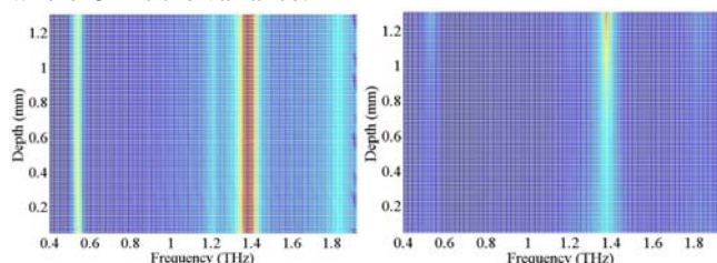
Fig.1 Comparison of the spectrograms for lactose sample
