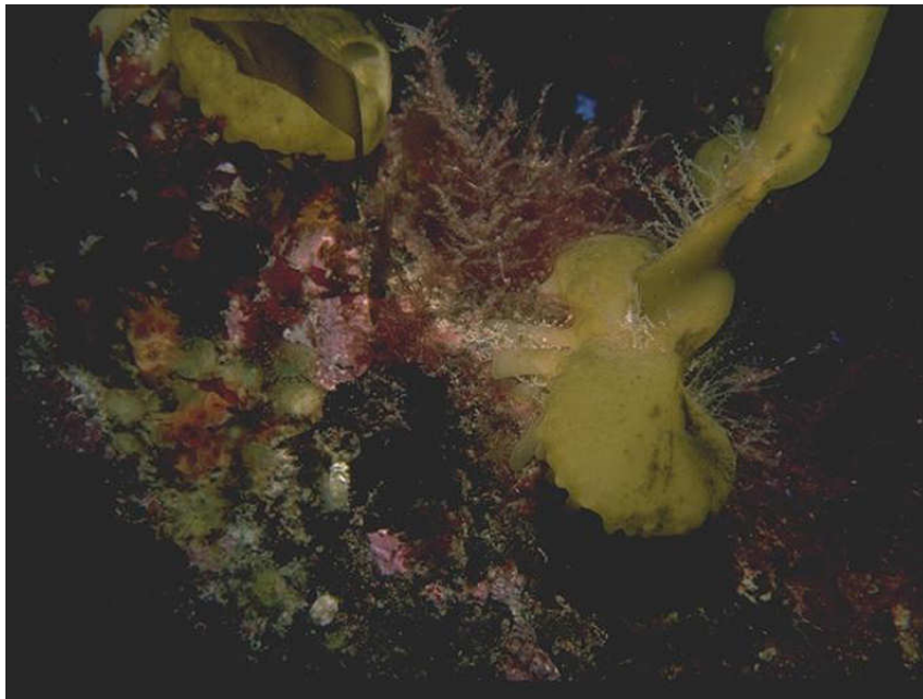
Saccharina latissima and/or Saccorhiza polyschides on exposed infralittoral rock.
