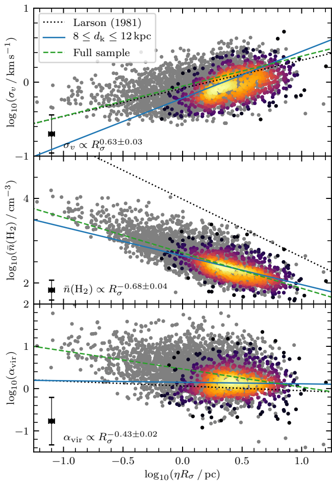
Fig. 10. Size–linewidth ( top panel ), size–density ( middle panel ), and size–virial parameter ( bottom panel ) relationships for the CHIMPS clumps, where the size parameter is the scaled intensity-weighted rms size (described in the text), \eta R_\sigma , for which \eta = 2.0 . In each case, the grey data points show the full sample, while the distance-limited sample is shown as colour-scaled data points, for which the lightest colours indicate the highest density of points. The blue lines show the best-fitted power-law for the distance-limited sample, for which we display the median error bars on the black data point in the lower-left corner. The dashed green lines show the best fits to the full sample. The relationships derived in Larson (1981) are shown as black dotted lines for reference, and have been rescaled to match these quantities. Full details of the fits are given in Table 5.
