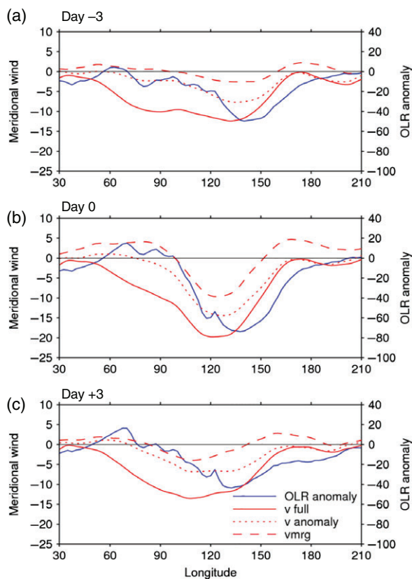
FIGURE 15 Fields at (a) day -3 , (b) day 0 and (c) day +3 of OLR ( 0\text{--}20^\circ\text{N} ) and near-equatorial v ( 5^\circ\text{N}\text{--}5^\circ\text{S} ) for the 30-year data for regressions on OLR in the WP region. Shown are the OLR anomaly (blue), 150 hPa v (continuous red line), and its anomaly (dotted red line). Also shown is the component of 150 hPa equatorial v associated with the projection onto the n = 0 equatorial MRG wave structures at 150 hPa (dashed red line). See text for more details
