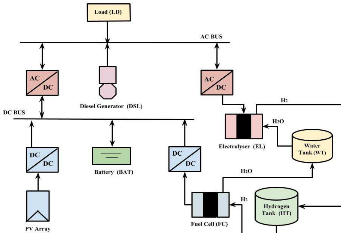
Fig. 1. Schematics of the experimental Islanded HESS [7] used as a case study
