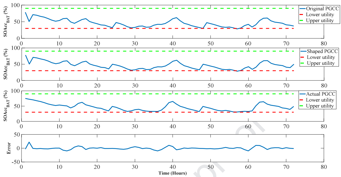
Fig 11. (a) The estimated and real Battery SOAcc response with the Kalman Adaptive PoPA for 72 h under Gaussian uncertainty; (b) converter logic
