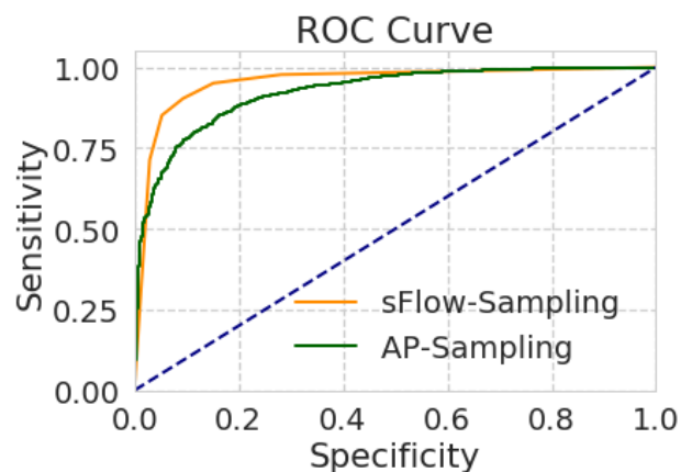
Figure 7: ROC Curve of 2 Class Classification.
