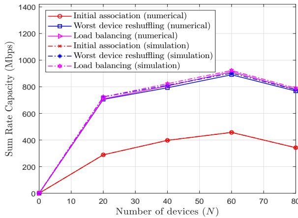
Fig. 5: Maximum sum rate vs number of SDs with both worst device reshuffling and load balancing techniques with k = 4 , l = 3 , and D = 0 .
