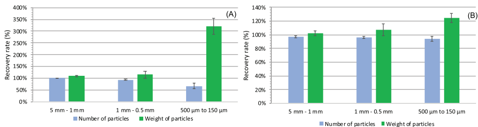
Fig. 4. Recovery results of spiked LDPE fragments by number of fragments (blue bars) and total weight of fragments (green bars). Panel A, 10 fragments; Panel B, 100 fragments. (Each value represents mean recovery from triplicate samples and bars indicate standard deviation).
