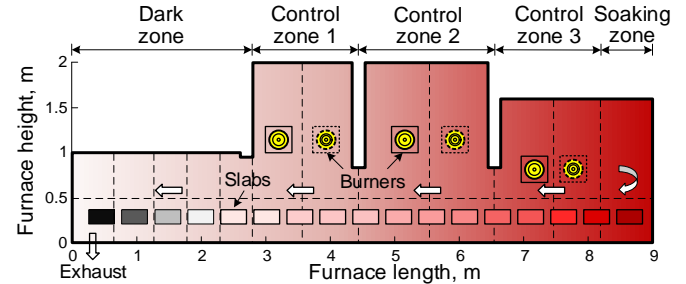
Figure 2. Outline of the pilot-scale reheating furnace
