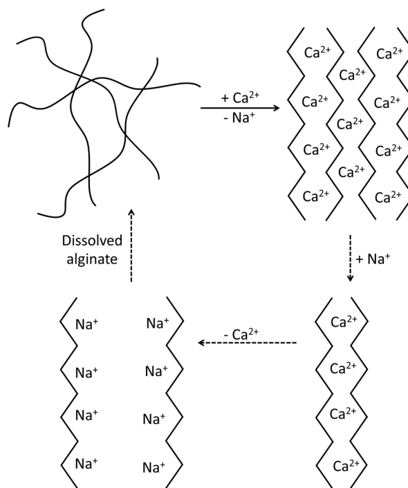
Figure 1: Egg-box model with expected ion transfer mechanism based on Ching et al. [9].
