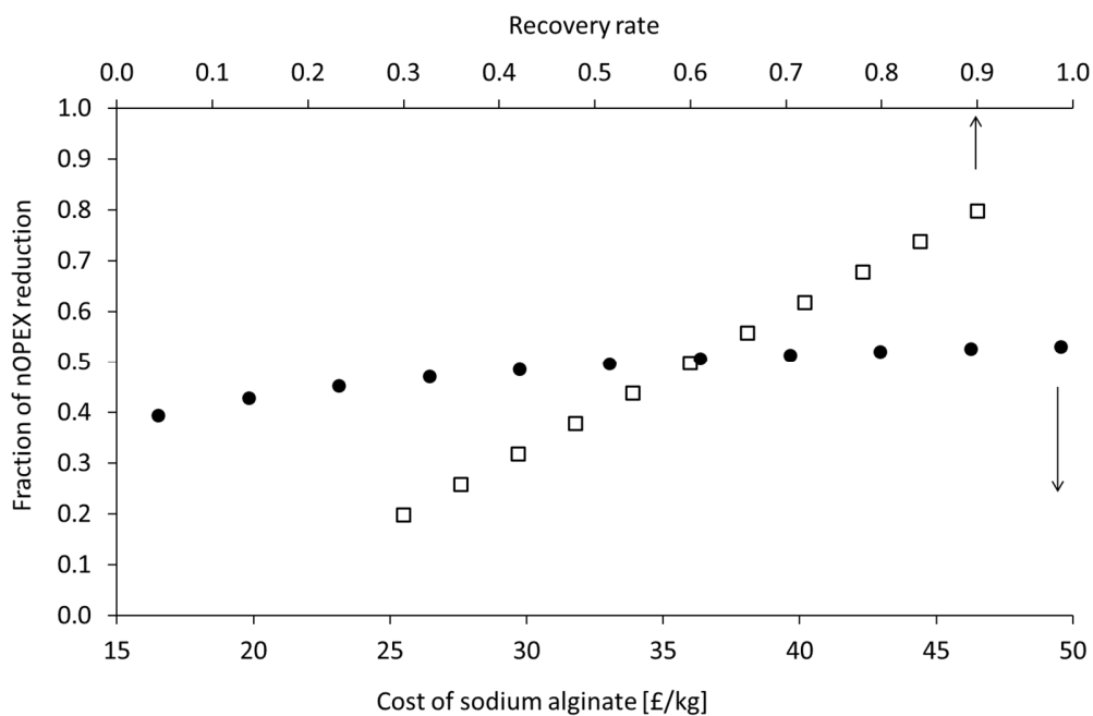
30 Figure 7: Development of nOPEX cost reduction with variation of sodium alginate costs 31 (●) and recovery rate (□).
