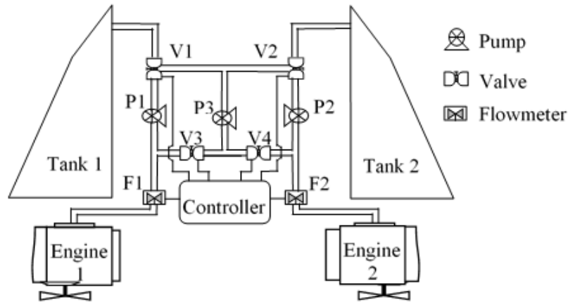
Figure 5: Fault tolerant fuel distribution system of a ship
