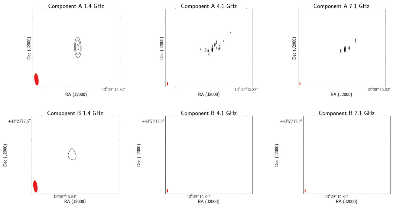
Figure A13. Multifrequency images of the lens candidate MJV16999 at 1.4 (left), 4.1 (centre), and 7.1 GHz (right). Component A is shown on the top row, and component B is shown on the bottom row. The beam is plotted in red on the bottom left corner of each image. Contour levels increase by a factor of 3, where the first contour is 3 times the off-source noise level and the cutouts are 0.08 \text{ arcsec} \times 0.08 \text{ arcsec} . The cutouts are centred at the coordinates listed in Table 2.
