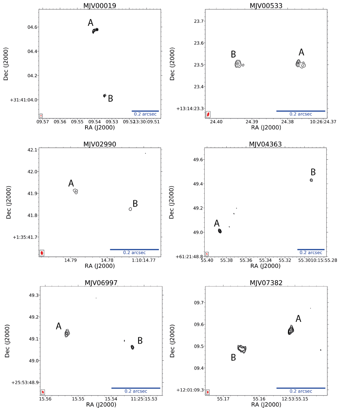
Figure 2. The CLEANed images at 1.4 GHz of the twelve lens candidates from the mJIVE-20 survey observations. Contours are at (-3, 3, 6, 9, 12, 15, 27) \times \sigma_{\text{rms}} , the off-source rms noise. The beam size is shown in the bottom left corner, which is on average 11 \times 5 \text{ mas}^2 ; north is up and east is left. The blue scale bar in each image represents 0.2 arcsec.
