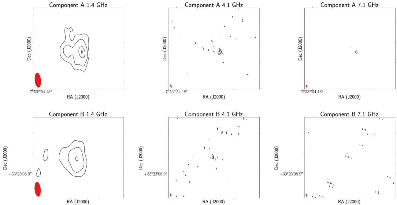
Figure A10. Multifrequency images of the lens candidate MJV11797 at 1.4 (left), 4.1 (centre), and 7.1 GHz (right). Component A is shown on the top row, component B is shown on the bottom row. The beam is plotted in red on the bottom left corner of each image. Contour levels increase by a factor of 3, where the first contour is three times the off-source noise level and the cutouts are 0.08 \text{ arcsec} \times 0.08 \text{ arcsec} . The cutouts are centred at the coordinates listed in Table 2.
