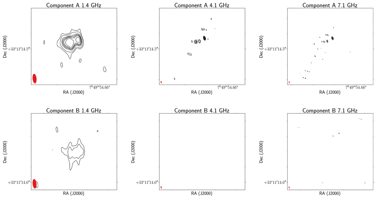
Figure A9. Multifrequency images of the lens candidate MJV11715 at 1.4 (left), 4.1 (centre), and 7.1 GHz (right). Component A is shown on the top row, and component B is shown on the bottom row. The beam is plotted in red on the bottom left corner of each image. Contour levels increase by a factor of 3, where the first contour is three times the off-source noise level and the cutouts are 0.1 \text{ arcsec} \times 0.1 \text{ arcsec} . The cutouts are centred at the coordinates listed in Table 2.
