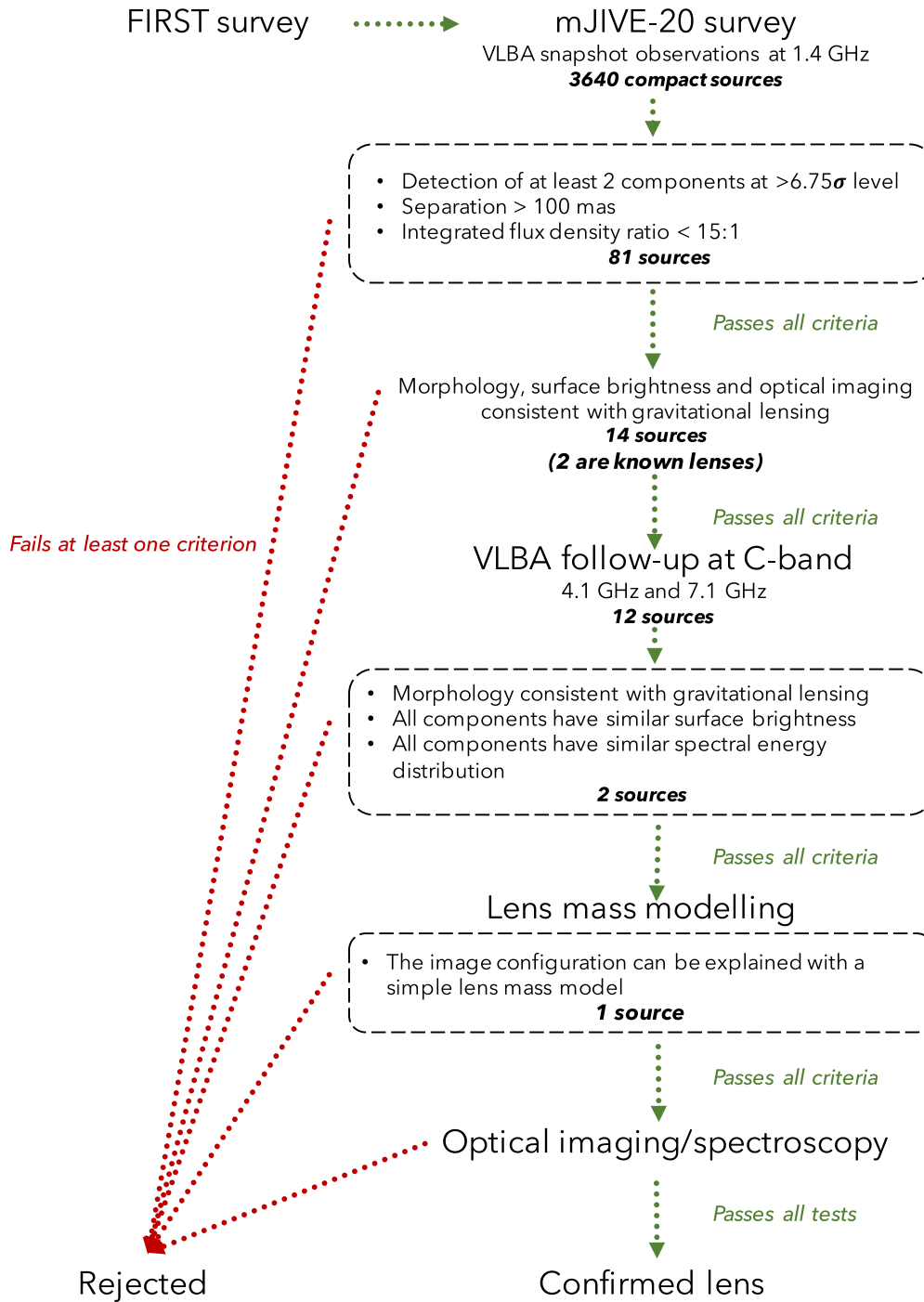
Figure 1. Flow chart diagram that summarizes the steps of the gravitational lensing search within the mJIVE-20 survey.
