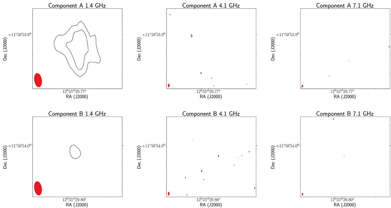
Figure A7. Multifrequency images of the lens candidate MJV07417 at 1.4 (left), 4.1 (centre), and 7.1 GHz (right). Component A is shown on the top row, and component B is shown on the bottom row. The beam is plotted in red on the bottom left corner of each image. Contour levels increase by a factor of 3, where the first contour is three times the off-source noise level and the cutouts are 0.08 \text{ arcsec} \times 0.08 \text{ arcsec} . The cutouts are centred at the coordinates listed in Table 2.
