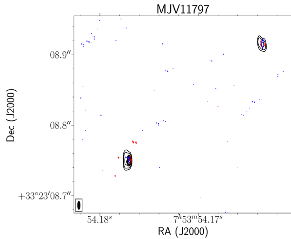
Figure A11. Overlay of contours at 1.7 GHz (black), 4.1 GHz (red), and 7.1 GHz (blue) of the lens candidate MJV11797 smoothed to a resolution of 12 \text{ mas} \times 3 \text{ mas} at PA of 0.150^\circ . The restoring beam is shown in the bottom left corner. The contour levels increase by a factor of 3, where the first contour is three times the off-source noise level.
