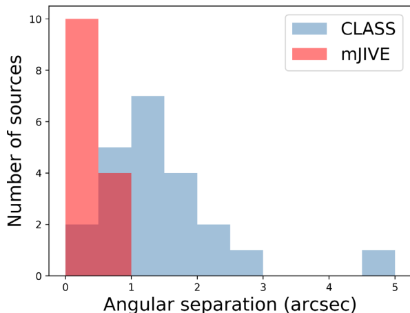
Figure 4. A comparison between the maximum image separation of the mJIVE-20 gravitational lens candidates (red) and the CLASS gravitational lenses (blue). The bins are 0.5 arcsec wide.
