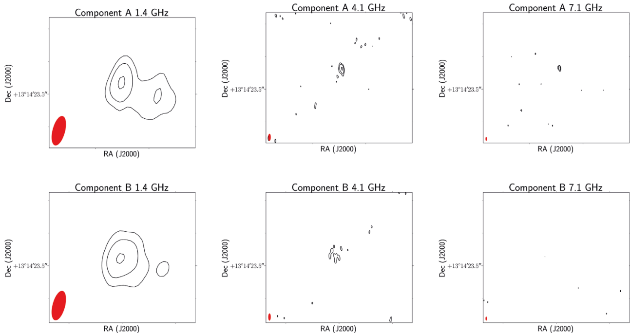
Figure A2. Multifrequency images of the lens candidate MJV00533 at 1.4 (left), 4.1 (centre), and 7.1 GHz (right). Component A is shown on the top row, and component B is shown on the bottom row. The beam is plotted in red on the bottom left corner of each image. Contour levels increase by a factor of 3, where the first contour is three times the off-source noise level and the cutouts are 0.08 \text{ arcsec} \times 0.08 \text{ arcsec} . The cutouts are centred at the coordinates listed in Table 2.
