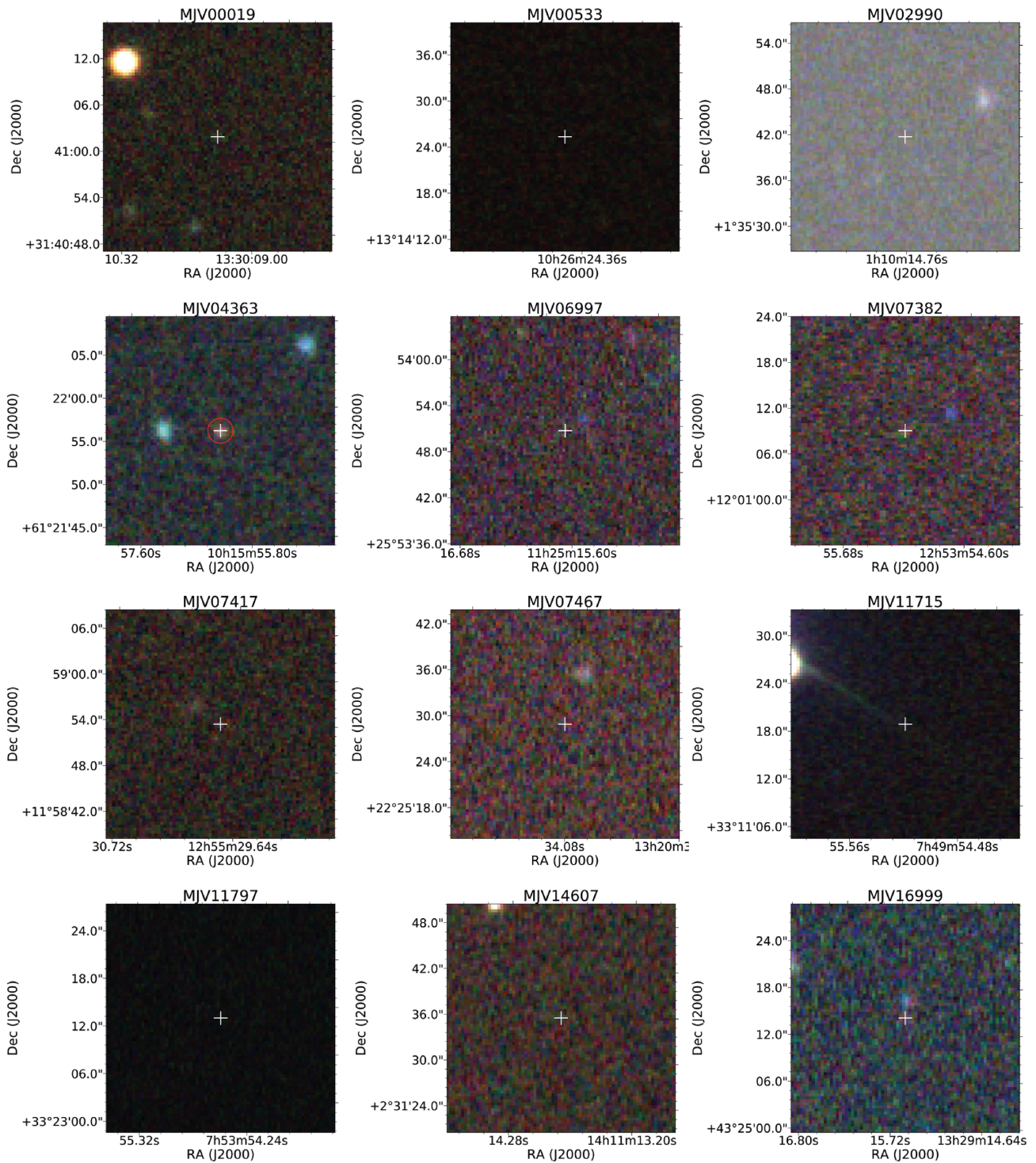
Figure A16. RGB SDSS images of the mJIVE-20 lens candidates. Cutouts are 0.5 \text{ arcmin} \times 0.5 \text{ arcmin} ; the white cross indicates the position of component A at 1.4 GHz, the red circle indicates the possible optical counterpart of the radio detection.
