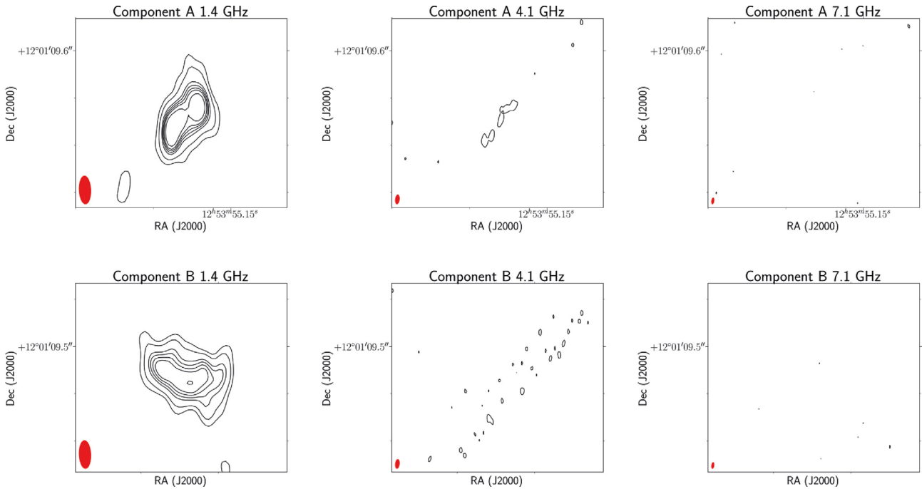
Figure A6. Multifrequency images of the lens candidate MJV07382 at 1.4 (left), 4.1 (centre), and 7.1 GHz (right). Component A is shown on the top row, and component B is shown on the bottom row. The beam is plotted in red on the bottom left corner of each image. Contour levels increase by a factor of 3, where the first contour is three times the off-source noise level and the cutouts are 0.08 \text{ arcsec} \times 0.08 \text{ arcsec} . The cutouts are centred at the coordinates listed in Table 2.
