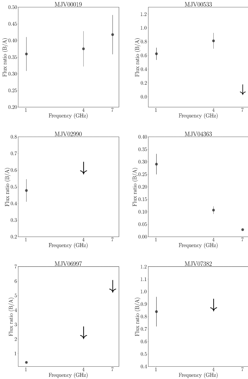
Figure A15. The flux density ratio ( B/A ) of the lens candidates as a function of frequency. The arrows represent the 3\sigma upper limits when a detection has been made of at least one candidate lensed image.
