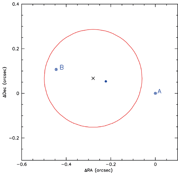
Figure 6. An SIS lens mass model that reproduces the image configuration of the candidate MJV07417. The observed positions are the open circles, while the model-predicted positions are indicated by the crosses. The critical curve is represented by the red solid line, and the black cross indicates the position of the lensing galaxy. The filled blue circle represents the source position.
