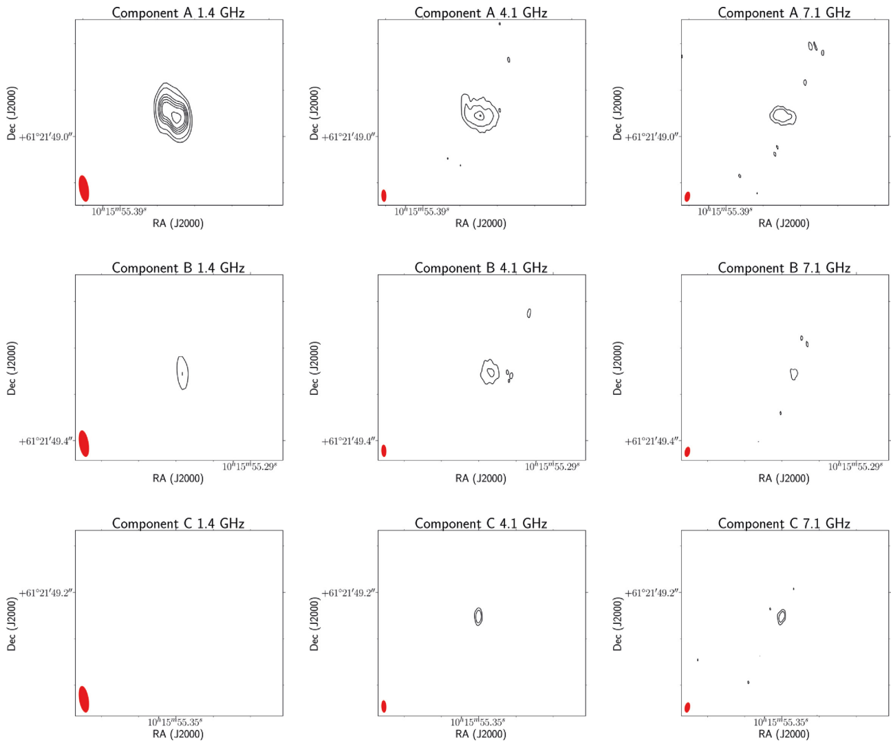
Figure A4. Multifrequency images of the lens candidate MJV04363 at 1.4 (left), 4.1 (centre), and 7.1 GHz (right). Component A is shown on the top row, and component B is shown on the second row and component C is shown on the bottom row. The beam is plotted in red on the bottom left corner of each image. Contour levels increase by a factor of 3, where the first contour is three times the off-source noise level and the cutouts are 0.08 \text{ arcsec} \times 0.08 \text{ arcsec} . The cutouts are centred at the coordinates listed in Table 2.
