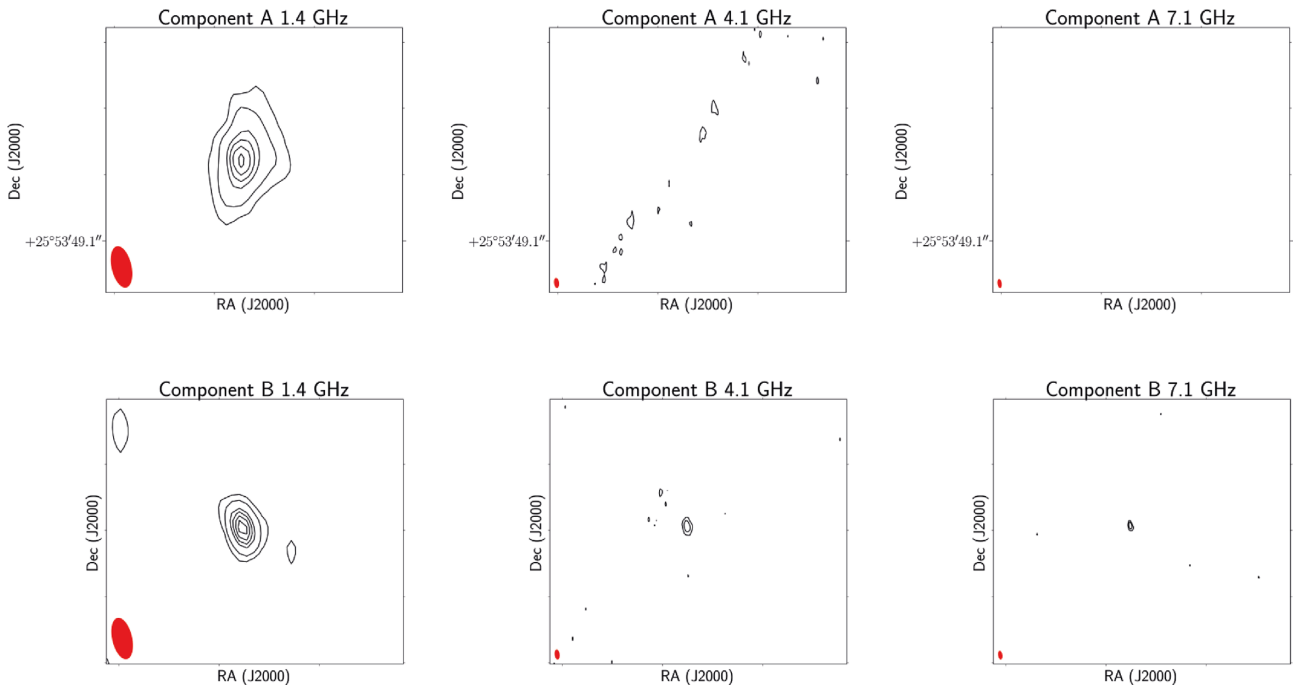
Figure A5. Multifrequency images of the lens candidate MJV06997 at 1.4 (left), 4.1 (centre), and 7.1 GHz (right). Component A is shown on the top row, and component B is shown on the bottom row. The beam is plotted in red on the bottom left corner of each image. Contour levels increase by a factor of 3, where the first contour is three times the off-source noise level and the cutouts are 0.08 \text{ arcsec} \times 0.08 \text{ arcsec} . The cutouts are centred at the coordinates listed in Table 2.
