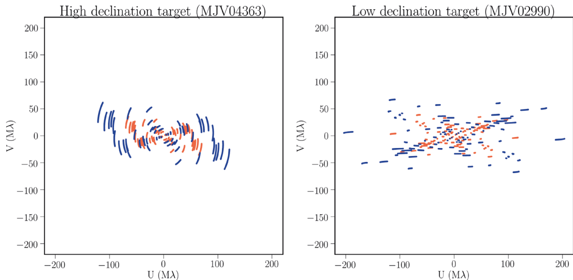
Figure 5. Examples of the uv -coverage for the highest (left) and lowest declination (right) lens candidates at 4.1 (orange points) and 7.1 GHz (blue points).
