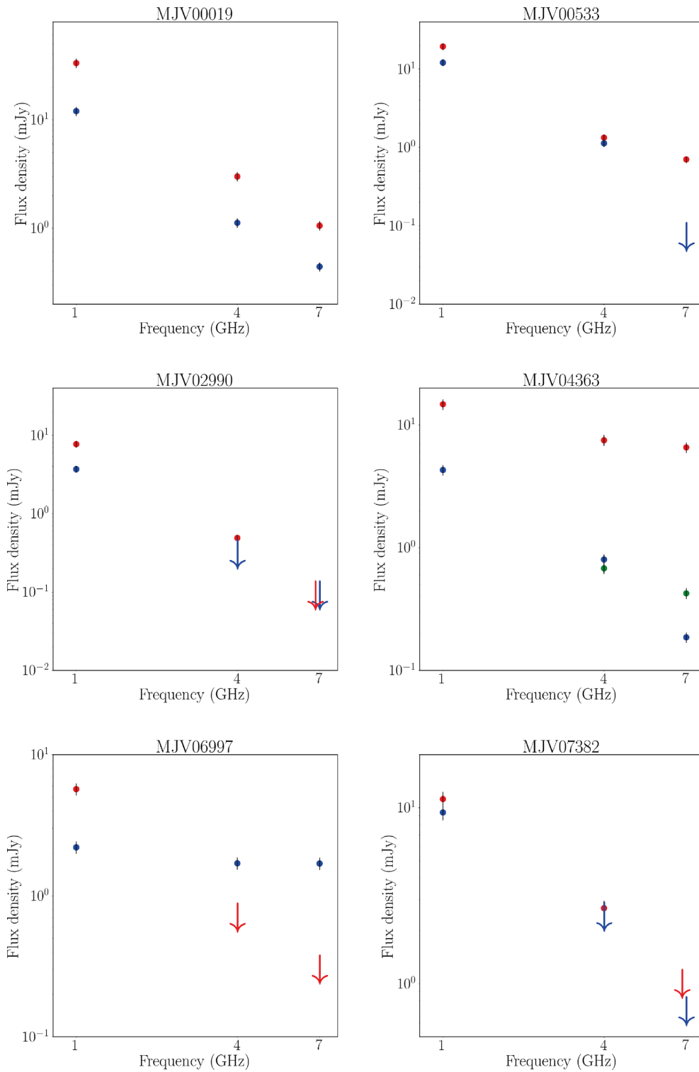
Figure A14. The spectral energy distribution of the lens candidates between 1.4 and 7.1 GHz. The filled circles indicate component A (red), B (blue) and, if detected, a third component C (green). The arrows indicate the 3\sigma detection limit at 4.1 and 7.1 GHz, estimated as three times the flux density within the same area of the 1.4 GHz detection of that image. The uncertainty on the flux density is assumed to be 10 per cent, which is a conservative estimate of the absolute flux density calibration of the VLBA.
