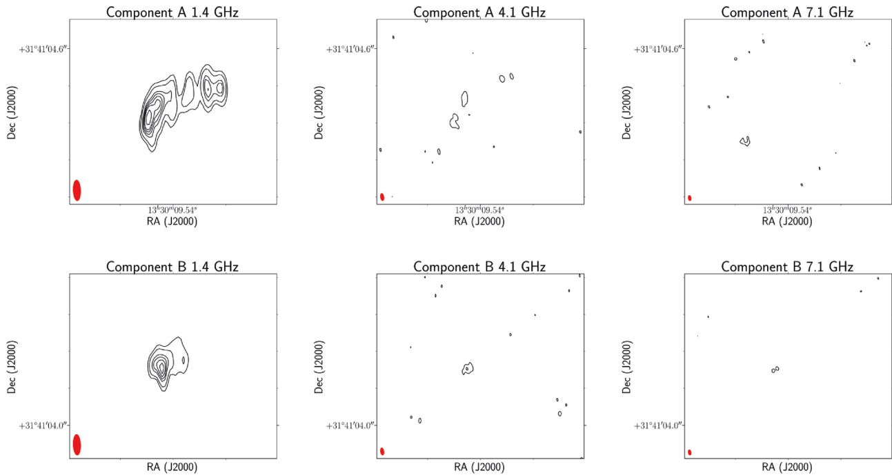
Figure A1. Multifrequency images of the lens candidate MJV00019 at 1.4 (left), 4.1 (centre), and 7.1 GHz (right). Component A is shown on the top row, and component B is shown on the bottom row. The beam is plotted in red on the bottom left corner of each image. Contour levels increase by a factor of 3, where the first contour is three times the off-source noise level and the cutouts are 0.08 \text{ arcsec} \times 0.08 \text{ arcsec} . The cutouts are centred at the coordinates listed in Table 2.
