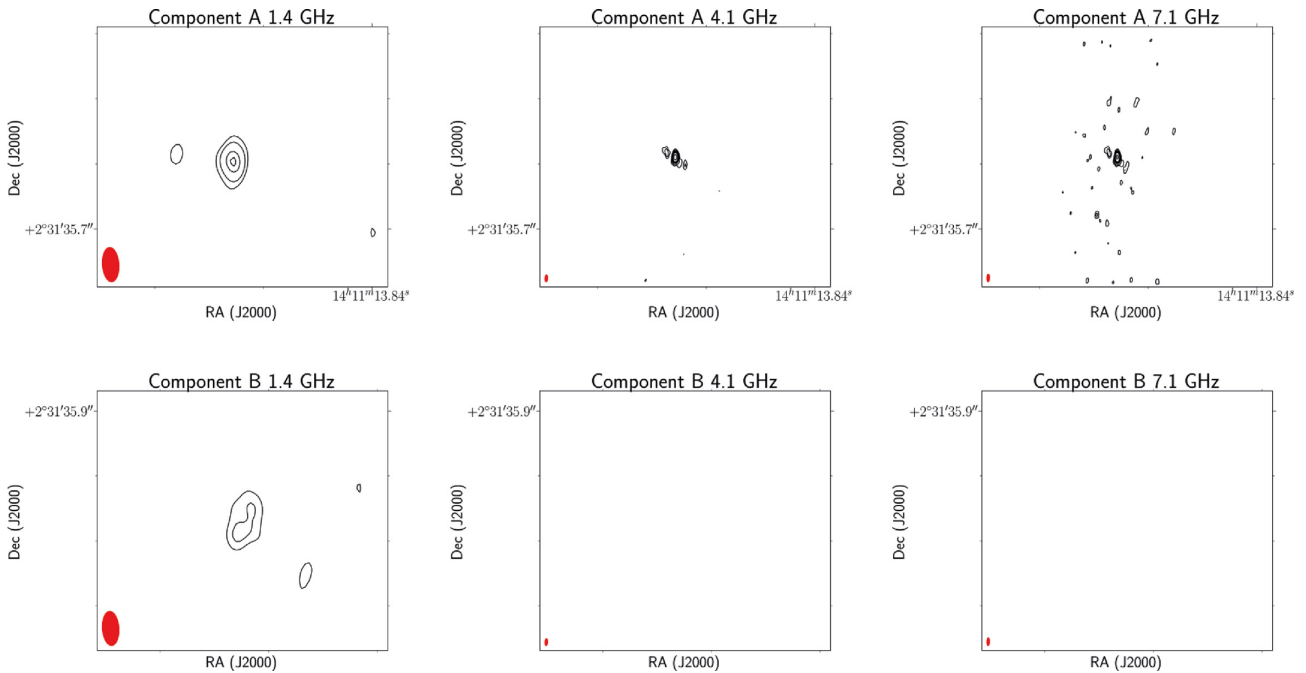
Figure A12. Multifrequency images of the lens candidate MJV14607 at 1.4 (left), 4.1 (centre), and 7.1 GHz (right). Component A is shown on the top row, and component B is shown on the bottom row. The beam is plotted in red on the bottom left corner of each image. Contour levels increase by a factor of 3, where the first contour is three times the off-source noise level and the cutouts are 0.08 \text{ arcsec} \times 0.08 \text{ arcsec} . The cutouts are centred at the coordinates listed in Table 2.
