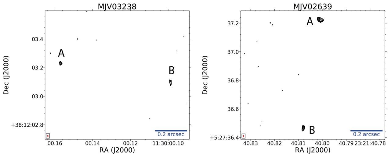
Figure 3. The self-calibrated images at 1.4 GHz of two mJIVE-20 sources that were previously confirmed as being gravitationally lensed by CLASS (B1127+385 is on the left and B2319+051 is on the right). Contours are at (-3, 3, 6, 9, 12, 15, 27) \times \sigma_{\text{rms}} , the off-source rms noise. The beam size is shown in the bottom left corner, which is on average 11 \times 5 \text{ mas}^2 ; north is up and east is left. The blue scale bar in each image represents 0.2 arcsec.
