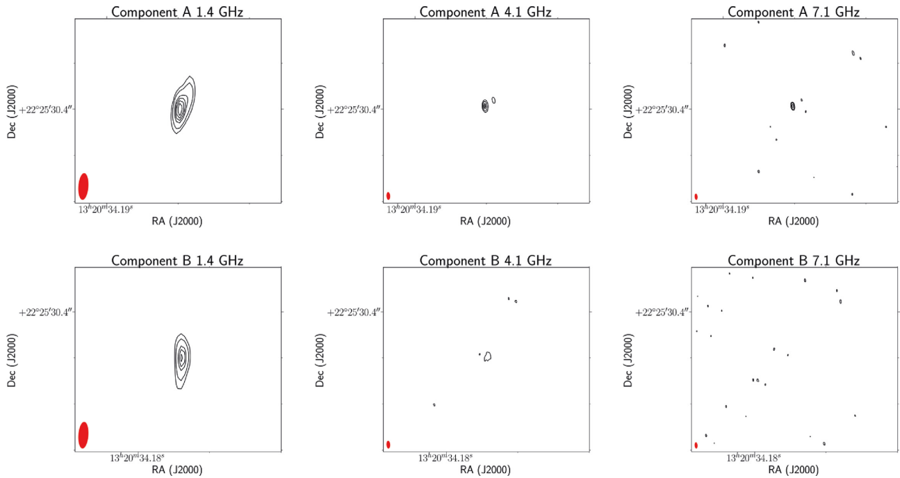
Figure A8. Multifrequency images of the lens candidate MJV07467 at 1.4 (left), 4.1 (centre), and 7.1 GHz (right). Component A is shown on the top row, and component B is shown on the bottom row. The beam is plotted in red on the bottom left corner of each image. Contour levels increase by a factor of 3, where the first contour is three times the off-source noise level and the cutouts are 0.08 \text{ arcsec} \times 0.08 \text{ arcsec} . The cutouts are centred at the coordinates listed in Table 2.
