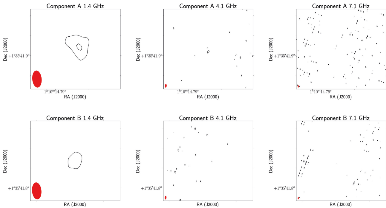
Figure A3. Multifrequency images of the lens candidate MJV02990 at 1.4 (left), 4.1 (centre), and 7.1 GHz (right). Component A is shown on the top row, and component B is shown on the bottom row. The beam is plotted in red on the bottom left corner of each image. Contour levels increase by a factor of 3, where the first contour is three times the off-source noise level and the cutouts are 0.08 \text{ arcsec} \times 0.08 \text{ arcsec} . The cutouts are centred at the coordinates listed in Table 2.
