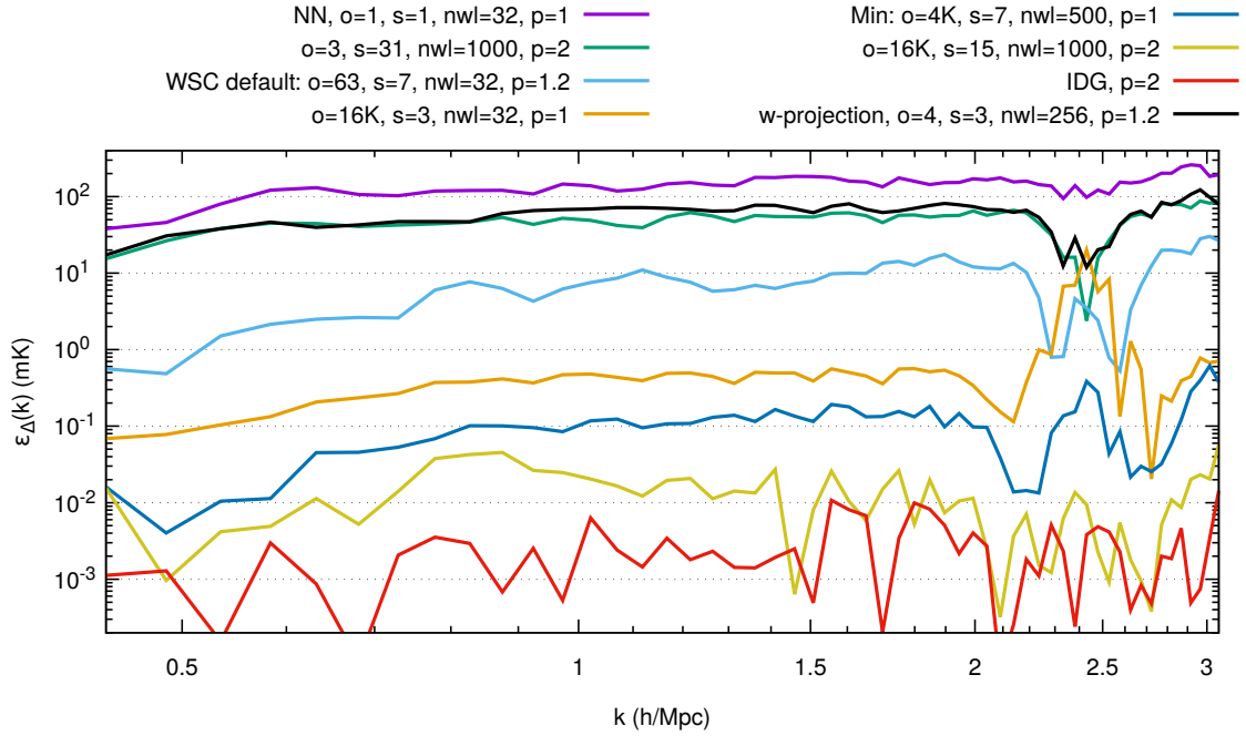
Fig. 2. Spherically averaged foreground-avoidance power spectra errors (absolute difference) without GPR foreground subtraction, compared to the directly Fourier transformed data. k values that fall under the wedge are excluded. Gridding parameters are abbreviated as follows: o = oversampling factor, s = gridding kernel size, nwl = number of w -layers, and p = padding factor.
